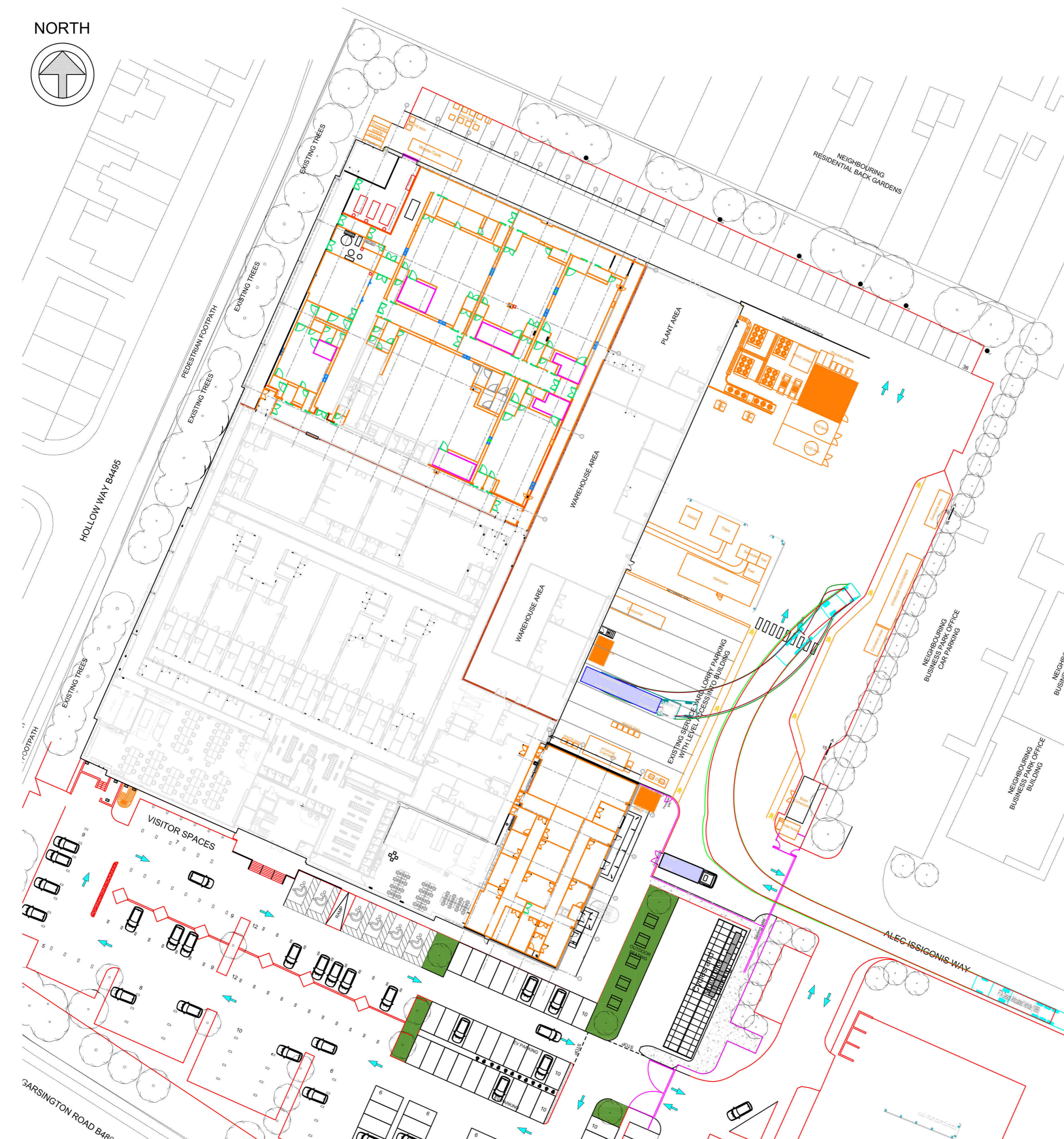
FTA Design Articulated Vehicle (Width 2.550m, length 16.480m) entering site
