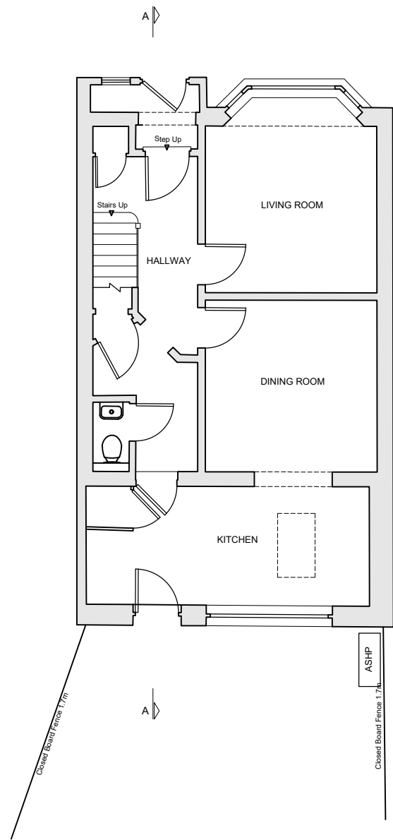
GROUND FLOOR - EXISTING
