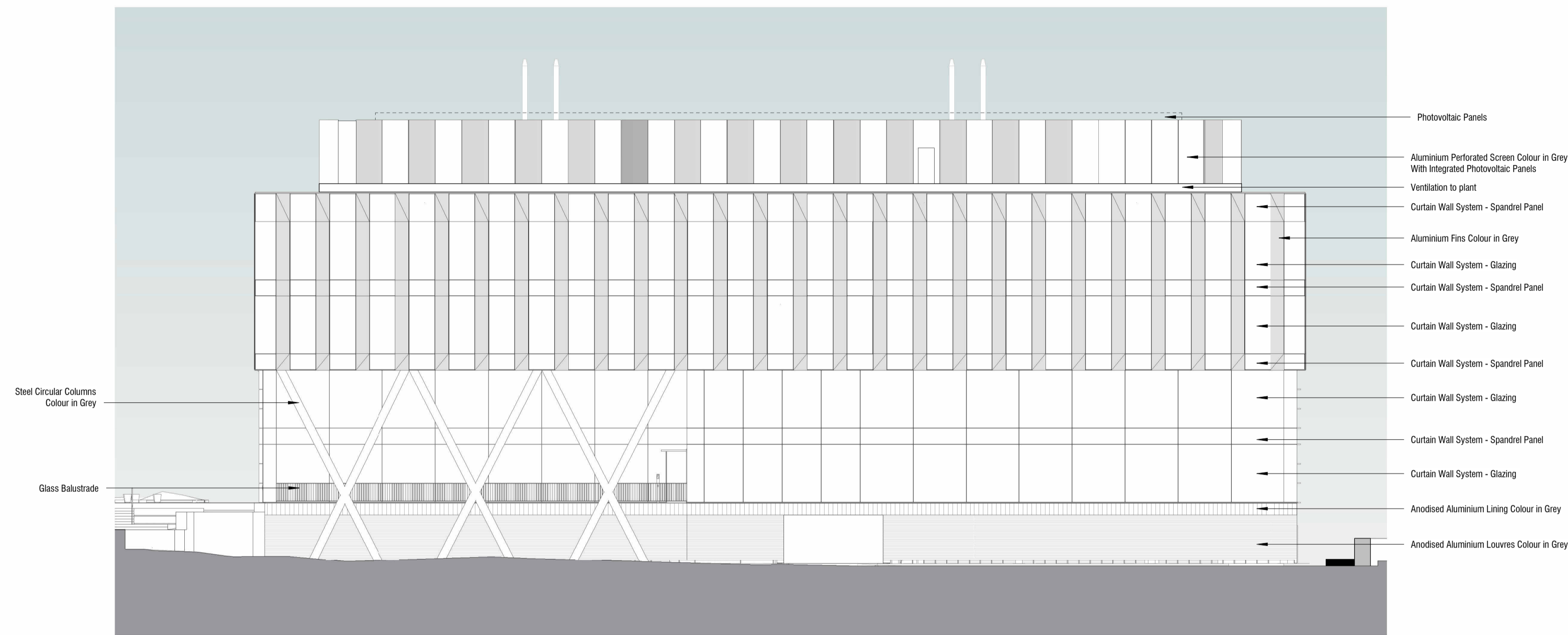
1 PROPOSED BUILDING 1 - NORTH EAST ELEVATION 1:200
