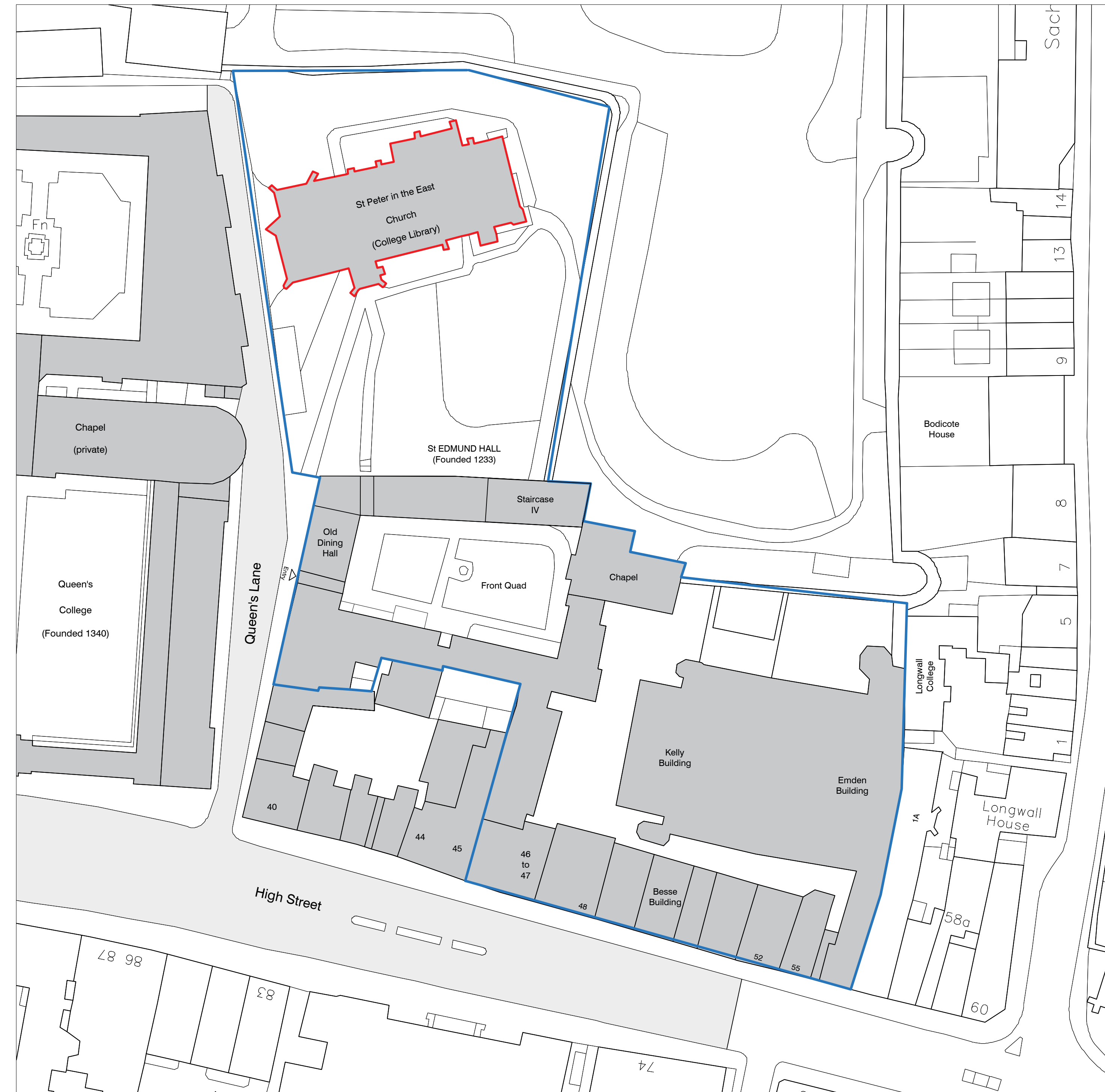
2 BLOCK PLAN 1:500
