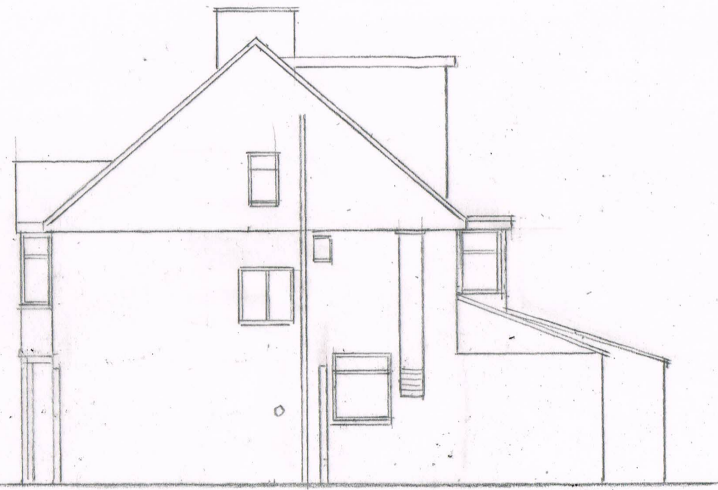
NORTH ELEVATION
