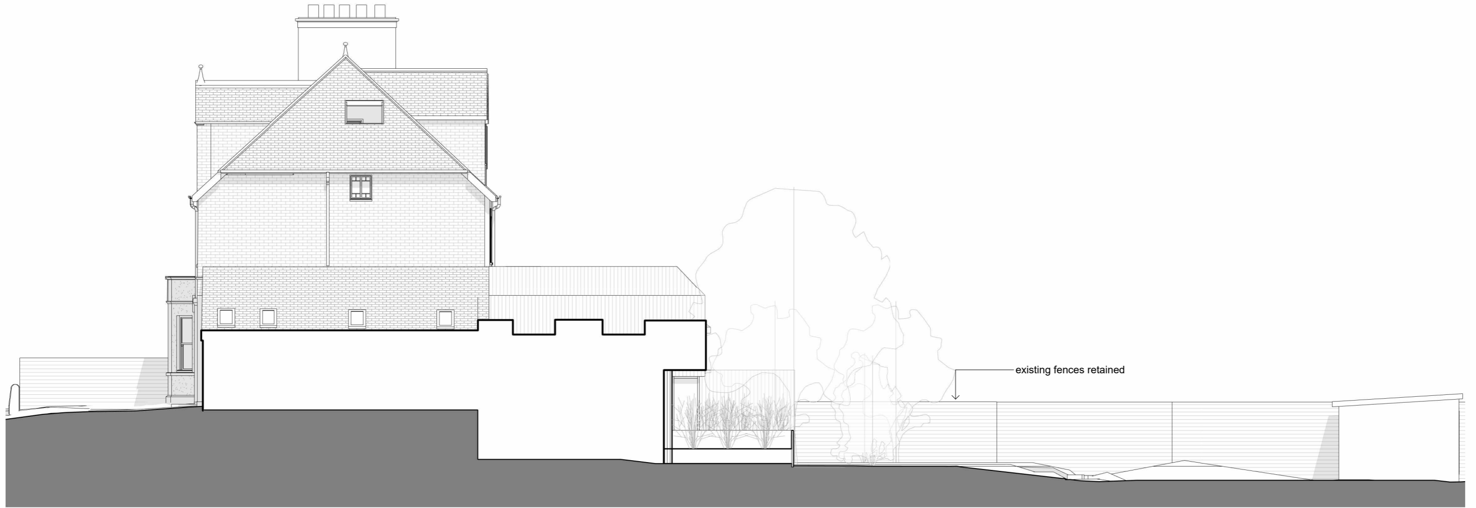
Proposed Elevation Looking South
