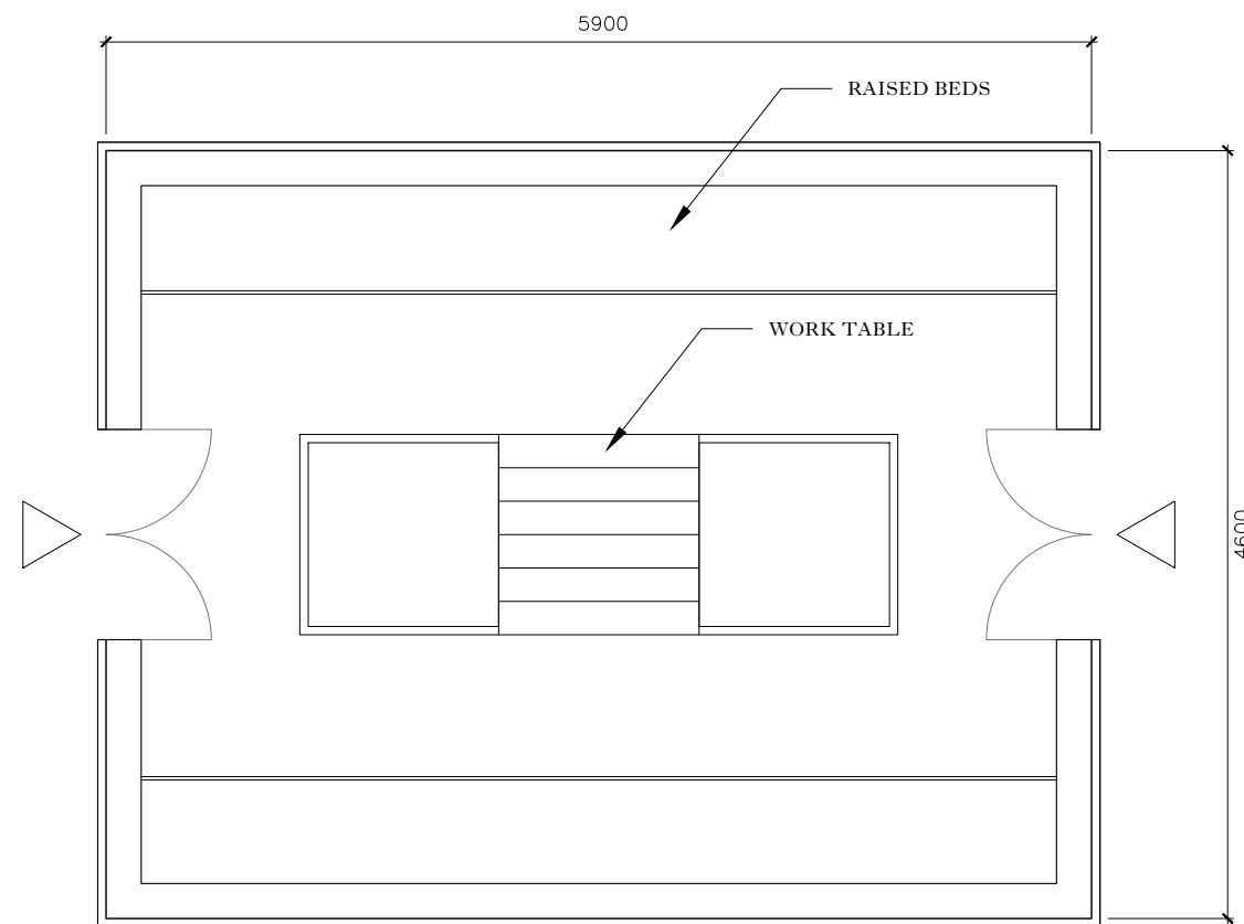
3 GREENHOUSE PLAN 1:50 @ A3
