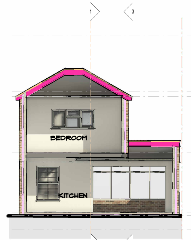
2 SECTION 2 SCALE 1 : 100 SHEET REF: Z3-A105
