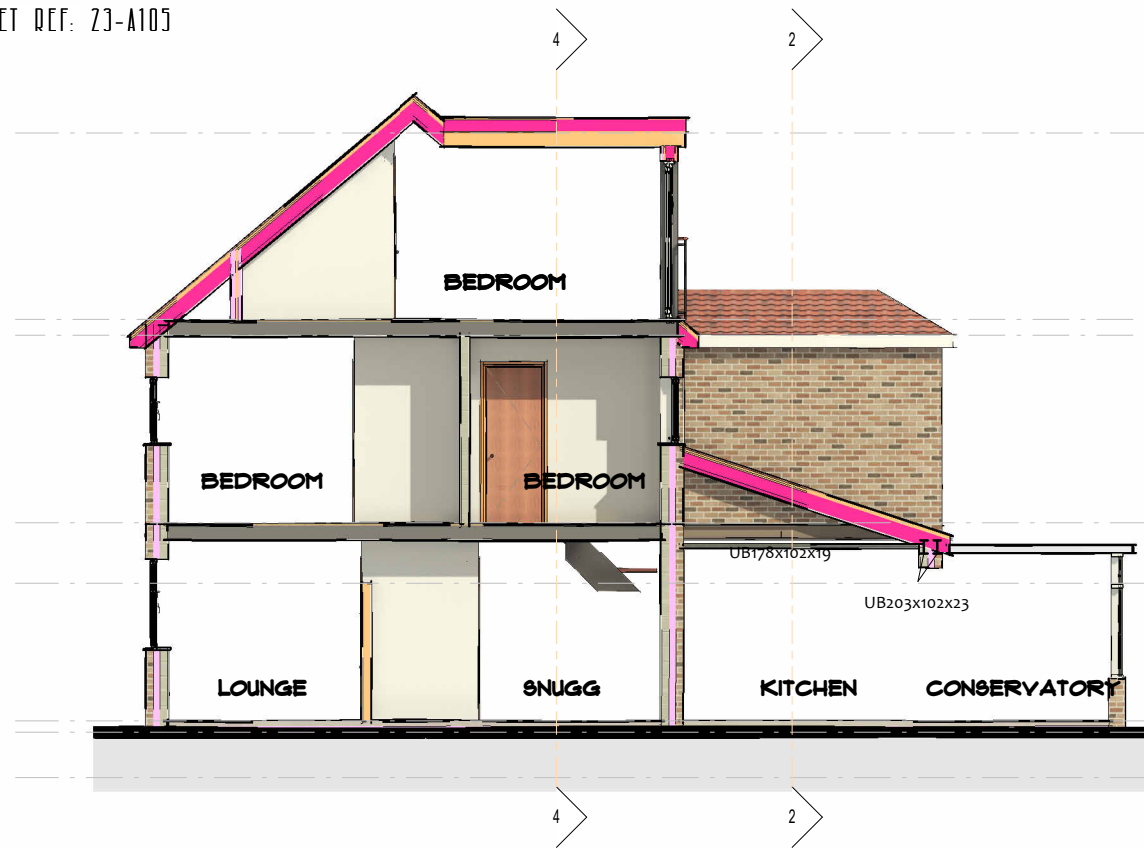
3 SECTION 3 SCALE 1 : 100 SHEET REF: Z3-A105
