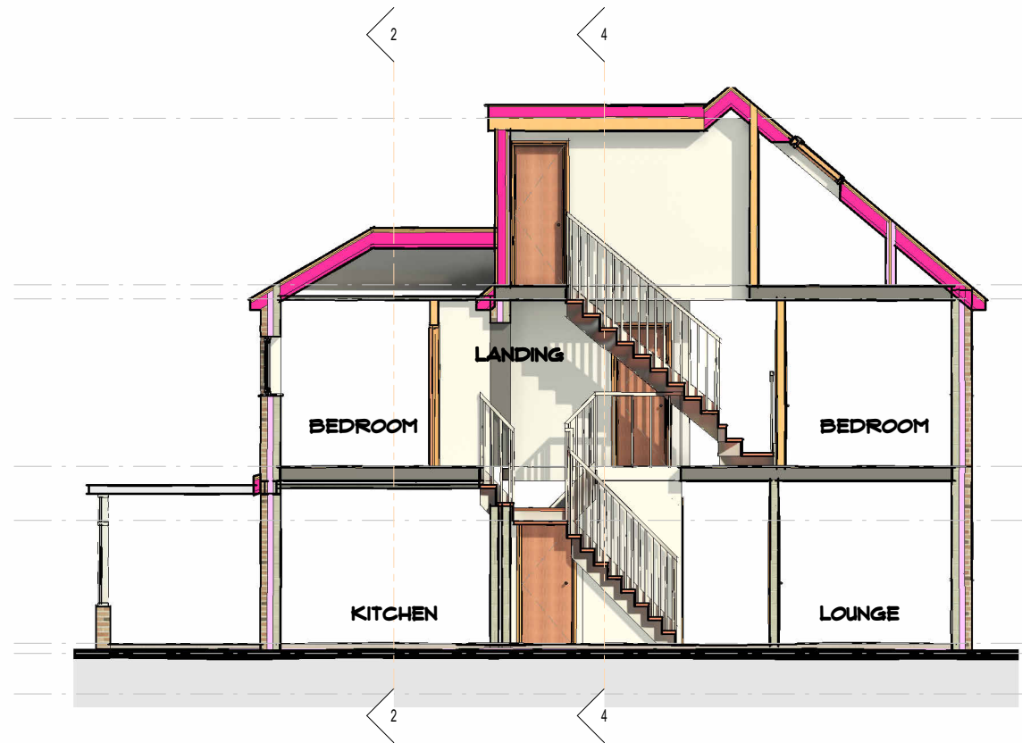
1 SECTION 1 SCALE 1 : 100 SHEET REF: Z3-A105
