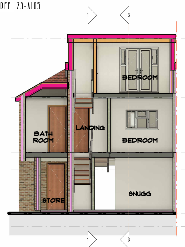
4 SECTION 4 SCALE 1 : 100 SHEET REF: Z3-A105
