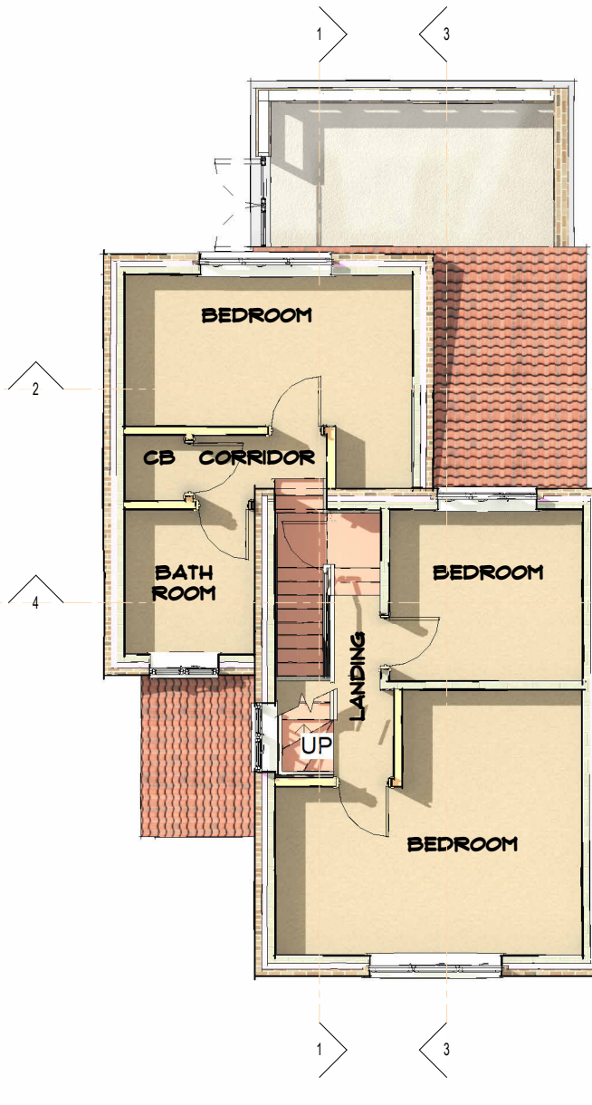
FF PRO. FIRST FLR. SCALE 1 : 100
