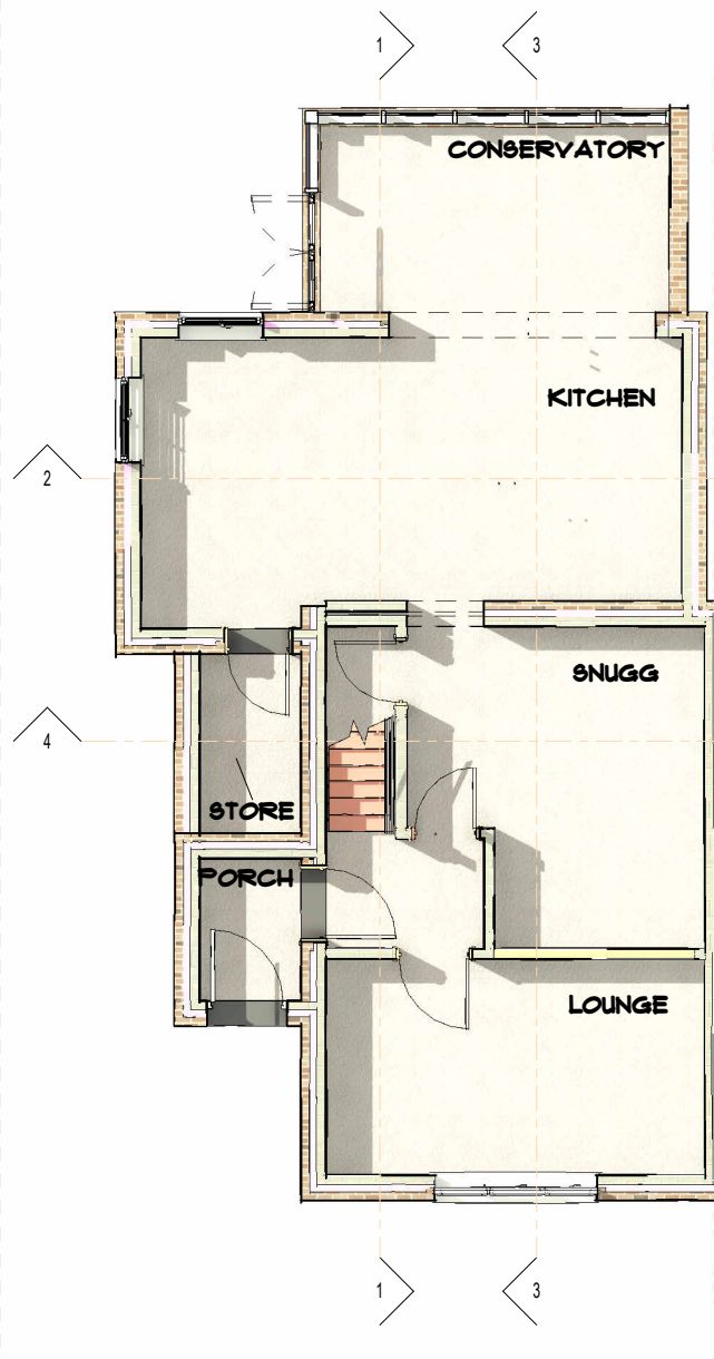
GF PRO. GROUND FLR. SCALE 1 : 100
