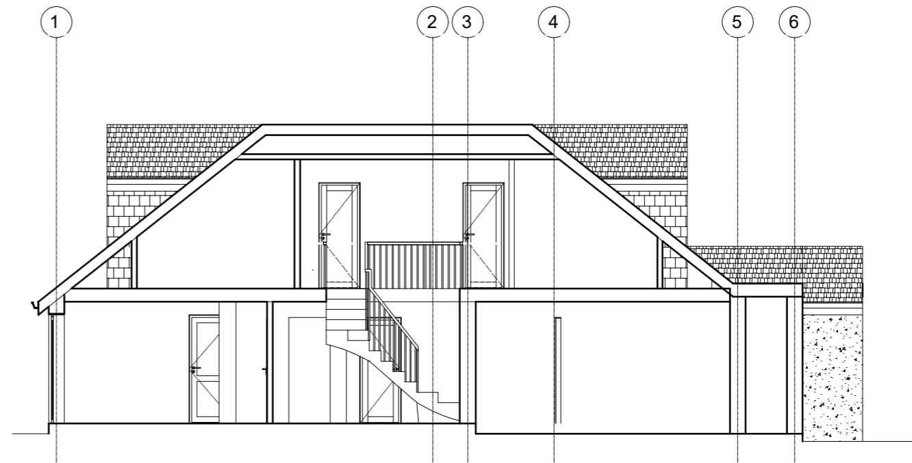
PROPOSED SECTION
