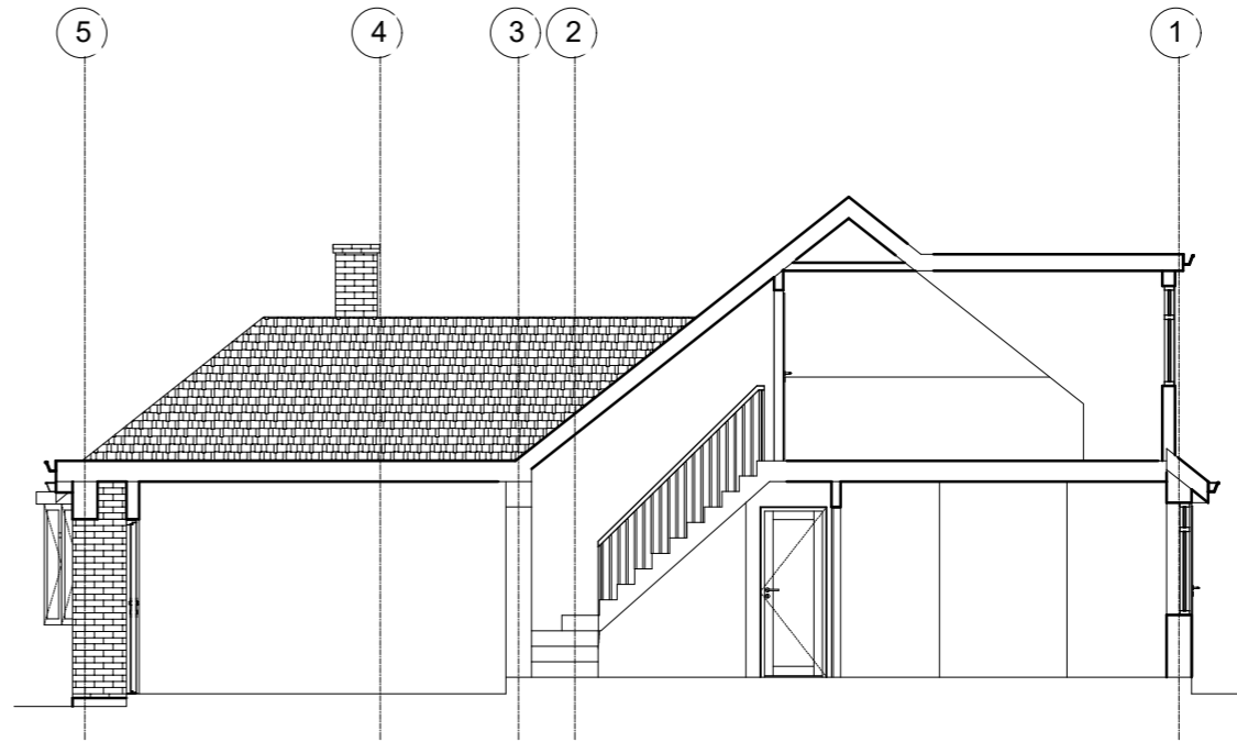
EXISTING SECTION
