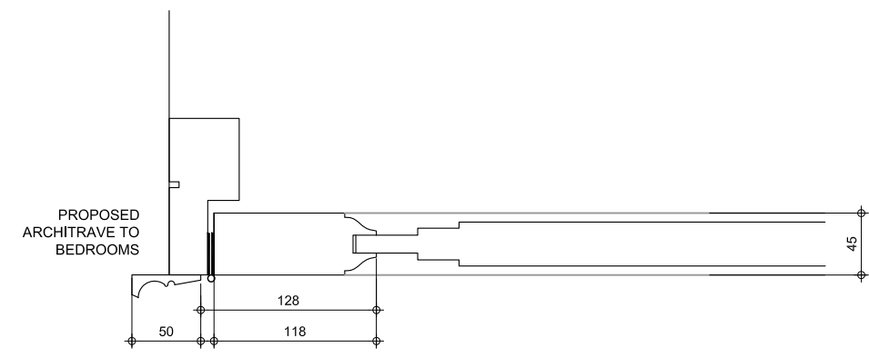
3 PROPOSED DOOR SECTION Scale: 1:5
