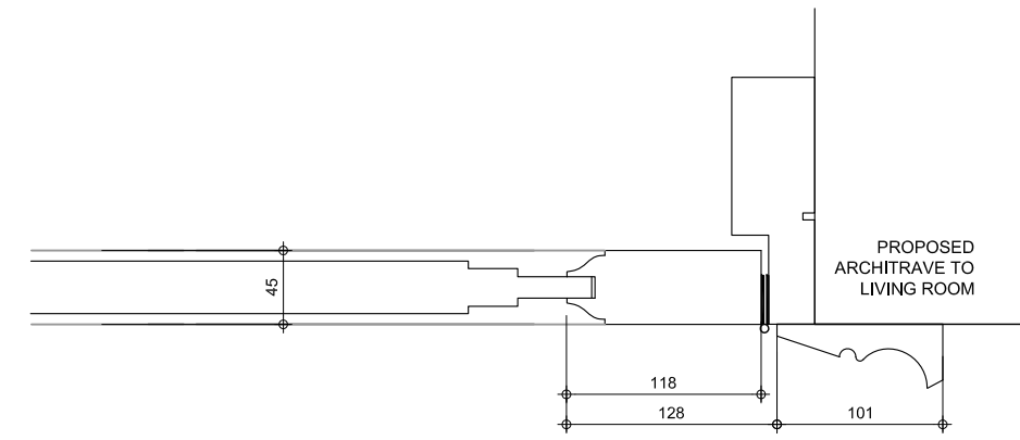
2 PROPOSED DOOR SECTION Scale: 1:5
