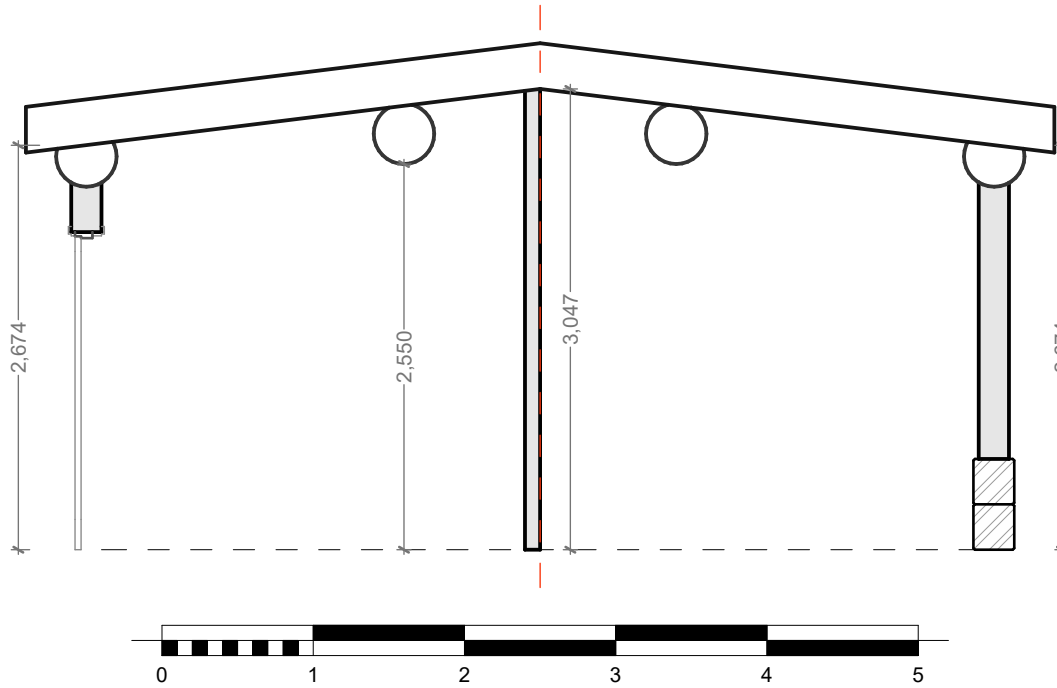
Cabin Section 1:50
