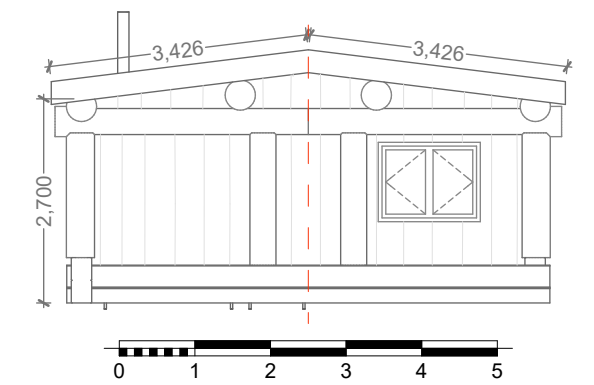
Right Elevation Cabin 1:100
