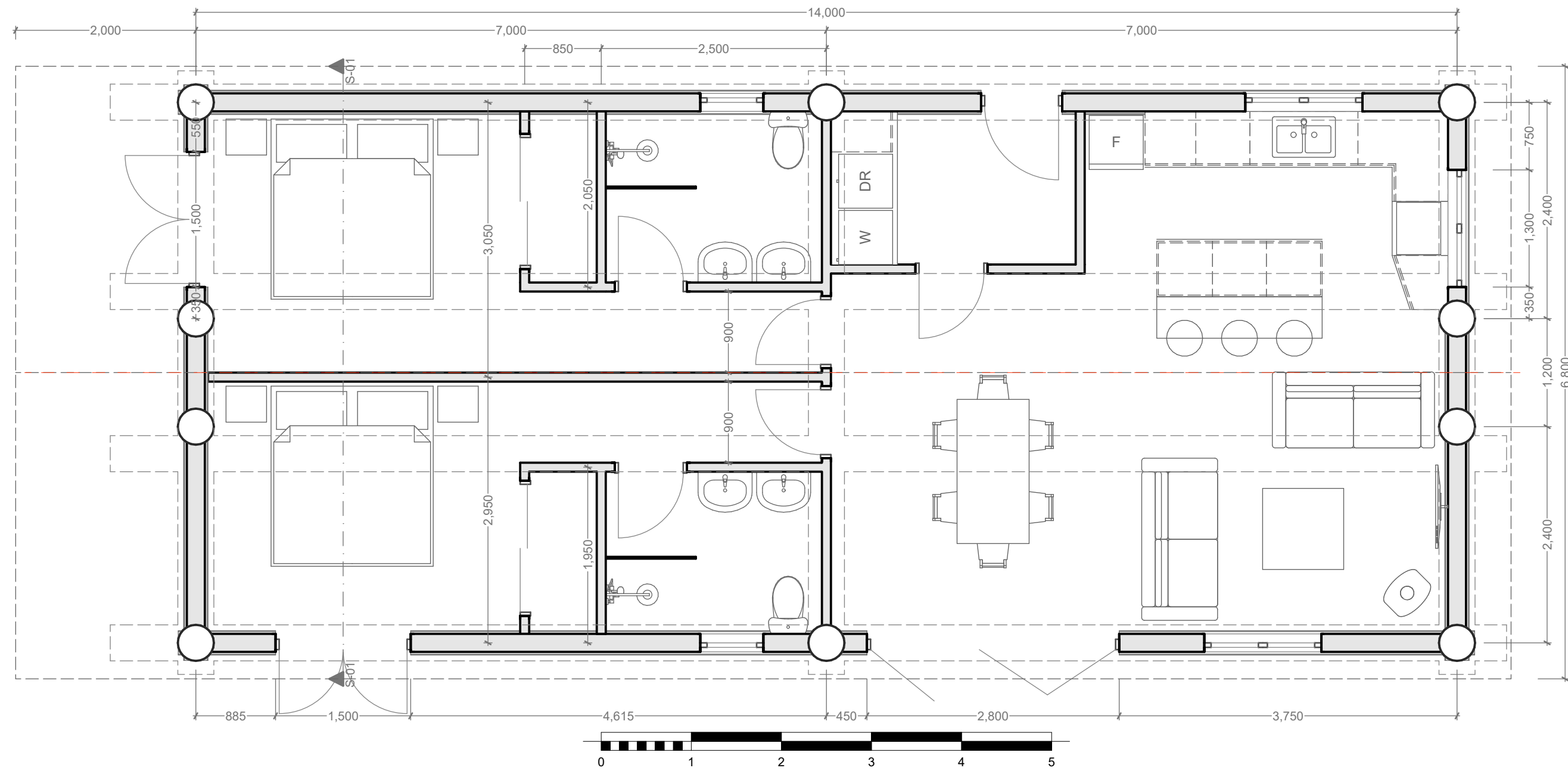
GF-Ground Floor Cabin 1:50
