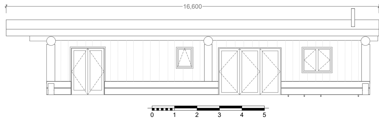
Front Elevation Cabin 1:100
