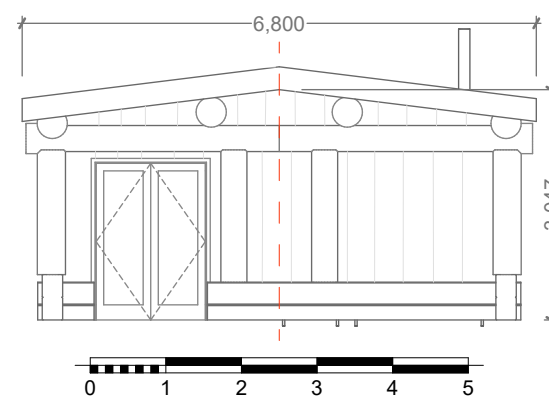
Left Elevation Cabin 1:100
