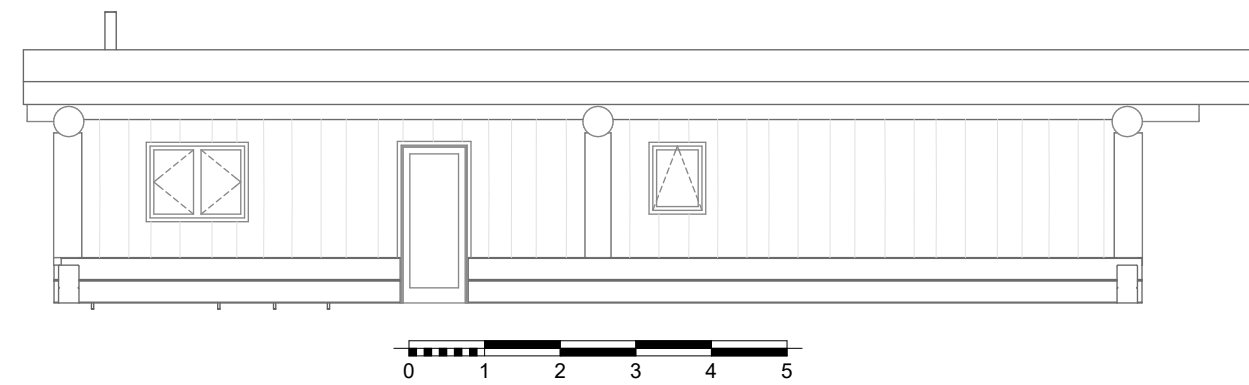
Rear Elevation Cabin 1:100
