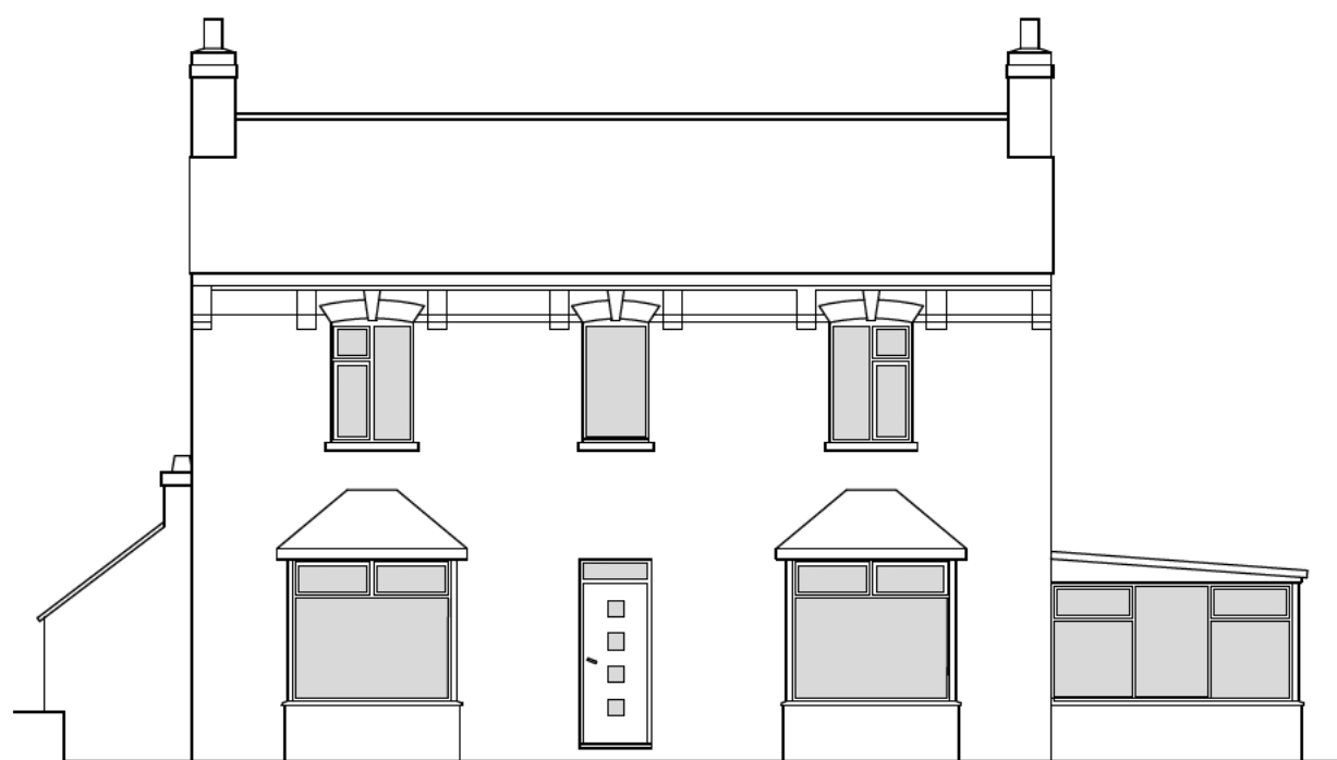
Existing South West Elevation
