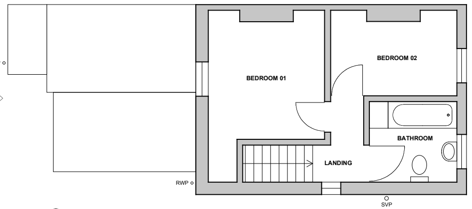
02 EXISTING FIRST FLOOR PLAN
