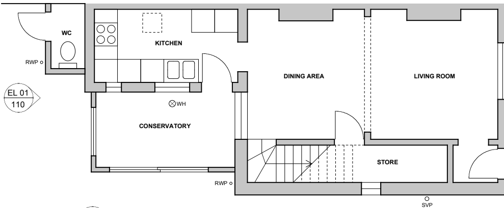
01 EXISTING GROUND FLOOR PLAN
