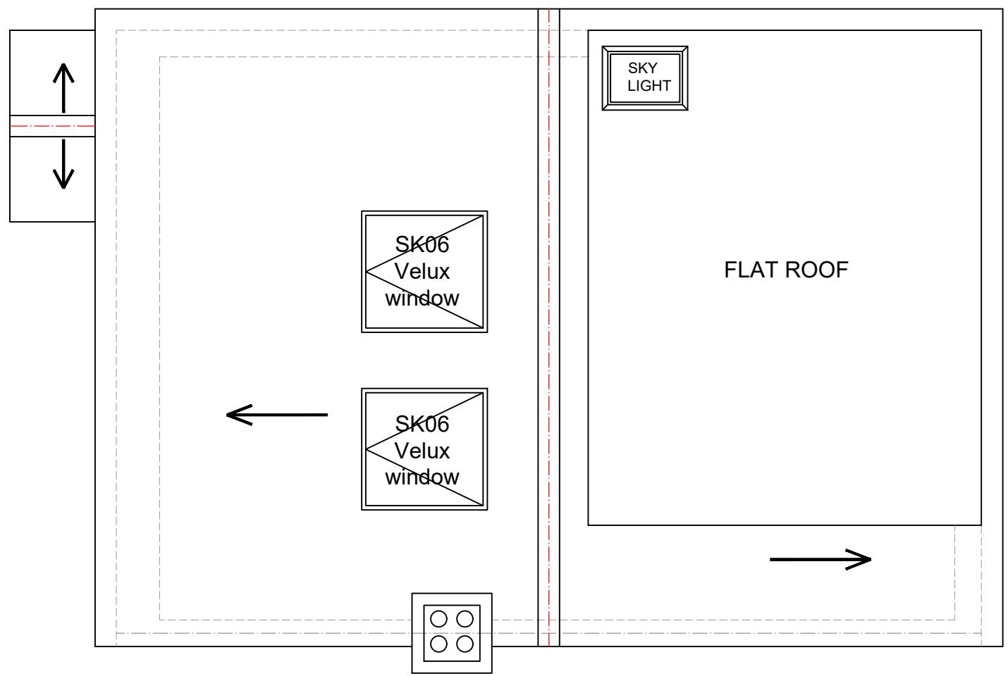
PROPOSED ROOF PLAN SCALE 1:50
