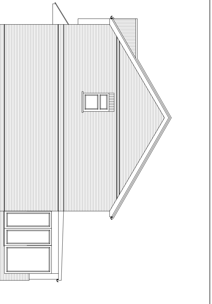
existing right side elevation
