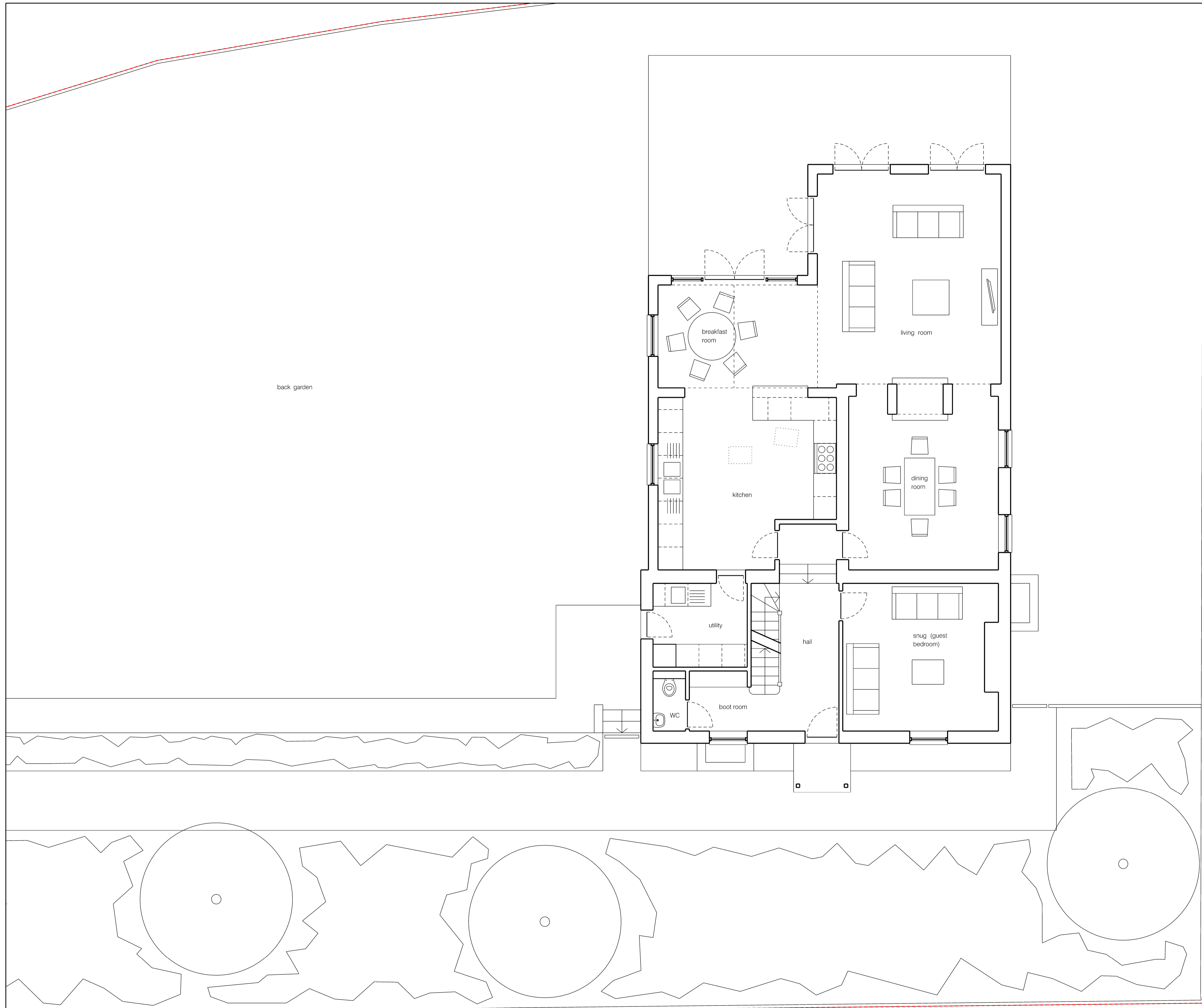
01 PROPOSED GROUND FLOOR PLAN
