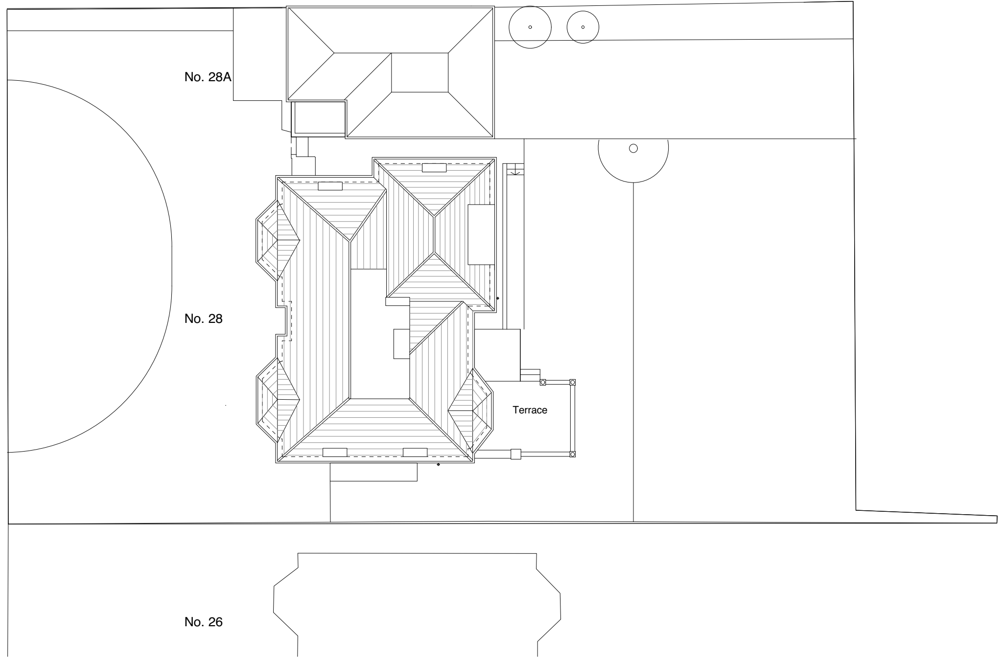
EXISTING SITE/ ROOF PLAN Scale 1:200
