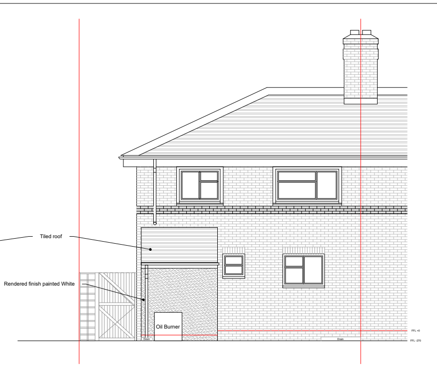
Northeast Elevation @1:100
