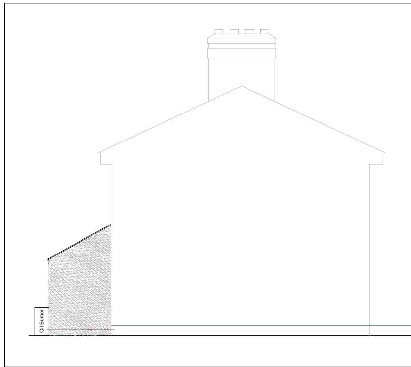
Northwest Elevation @1:100
