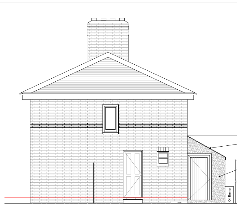
Southeast Elevation @ 1:100
