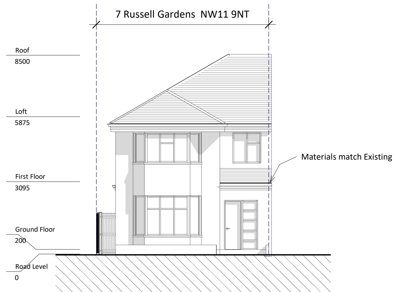
FRONT ELEVATION
