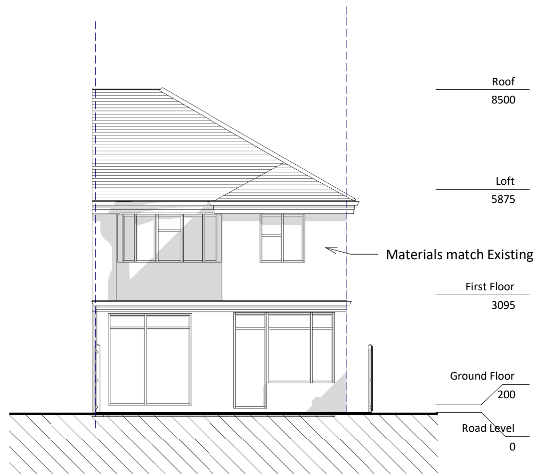
REAR ELEVATION
