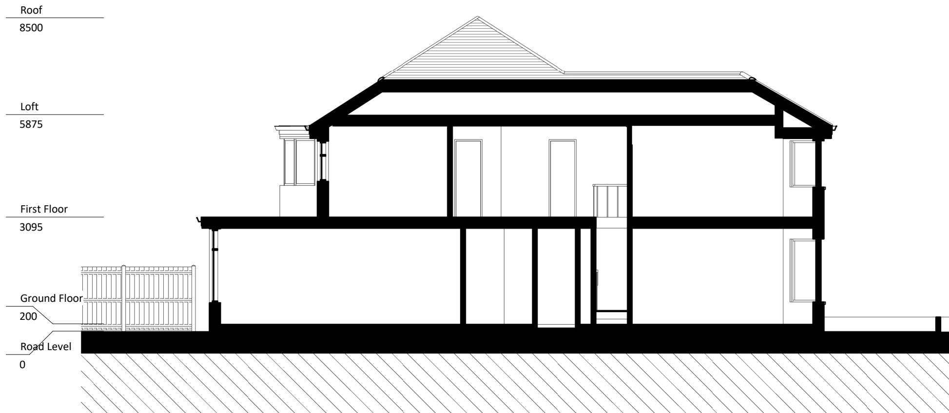
SECTION AA
