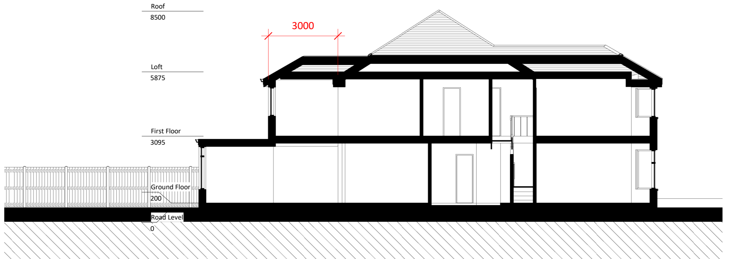
SECTION AA
