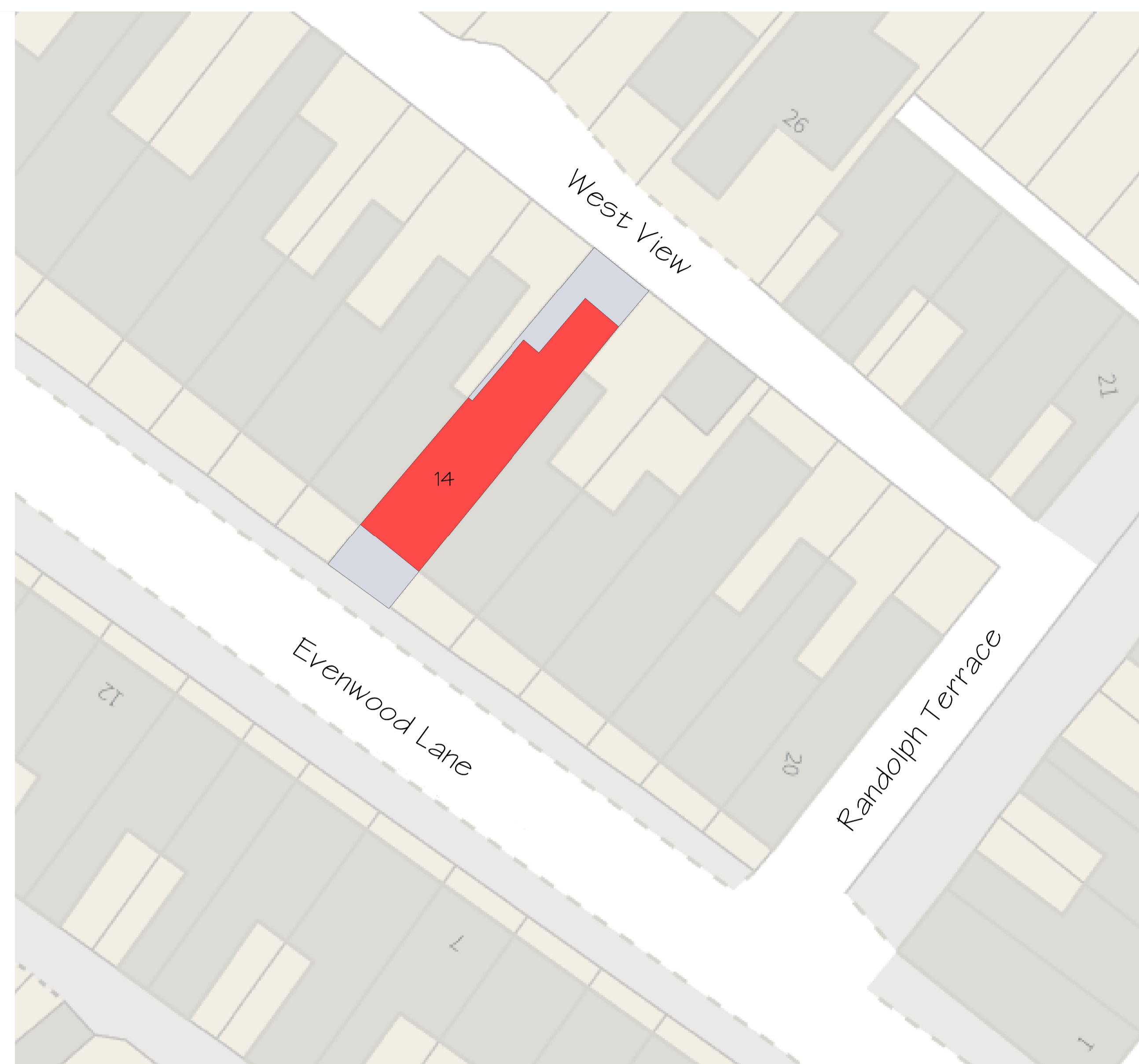
② Proposed Block Plan 1:200
