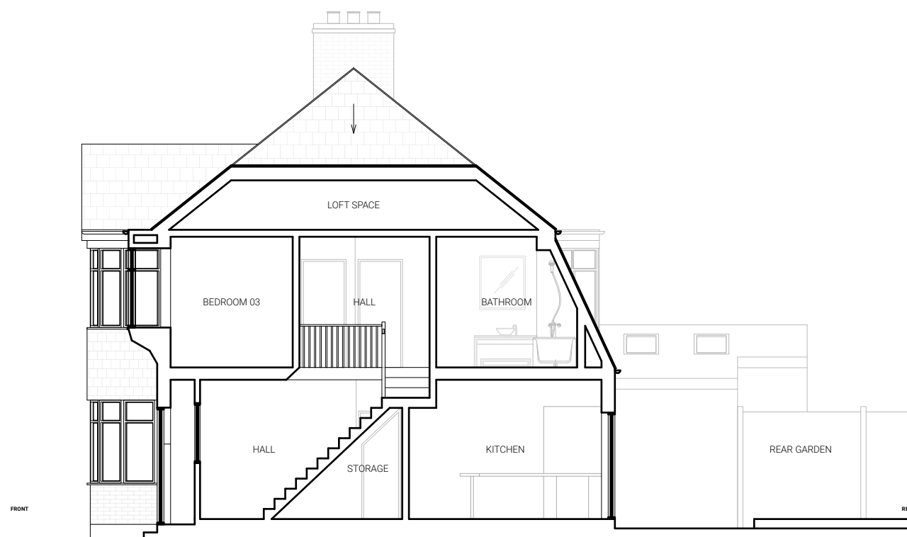
WEST SECTIONAL ELEVATION
