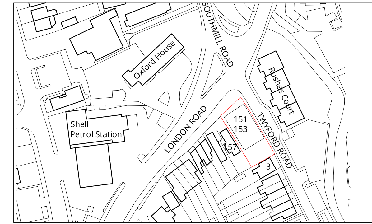
EXISTING LOCATION PLAN Scale 1:1250
