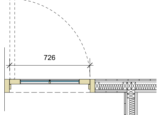
Door to Office D04 1:20 Plan
