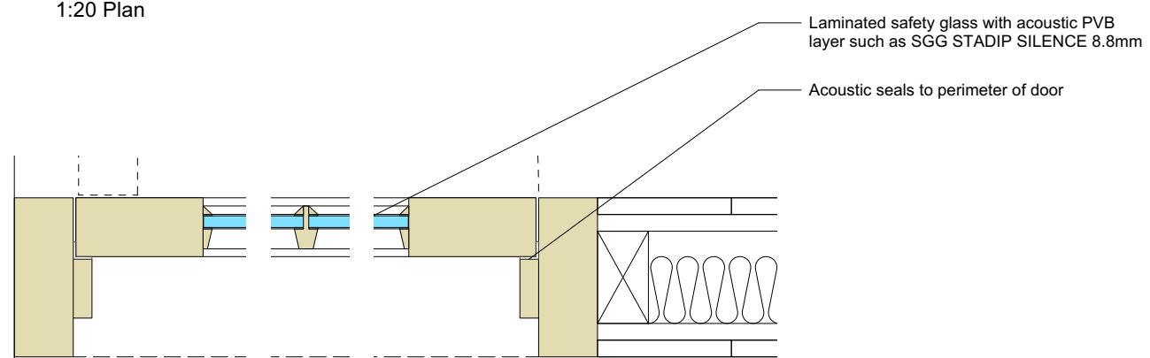
Door to Office D04 1:5 Plan Details
