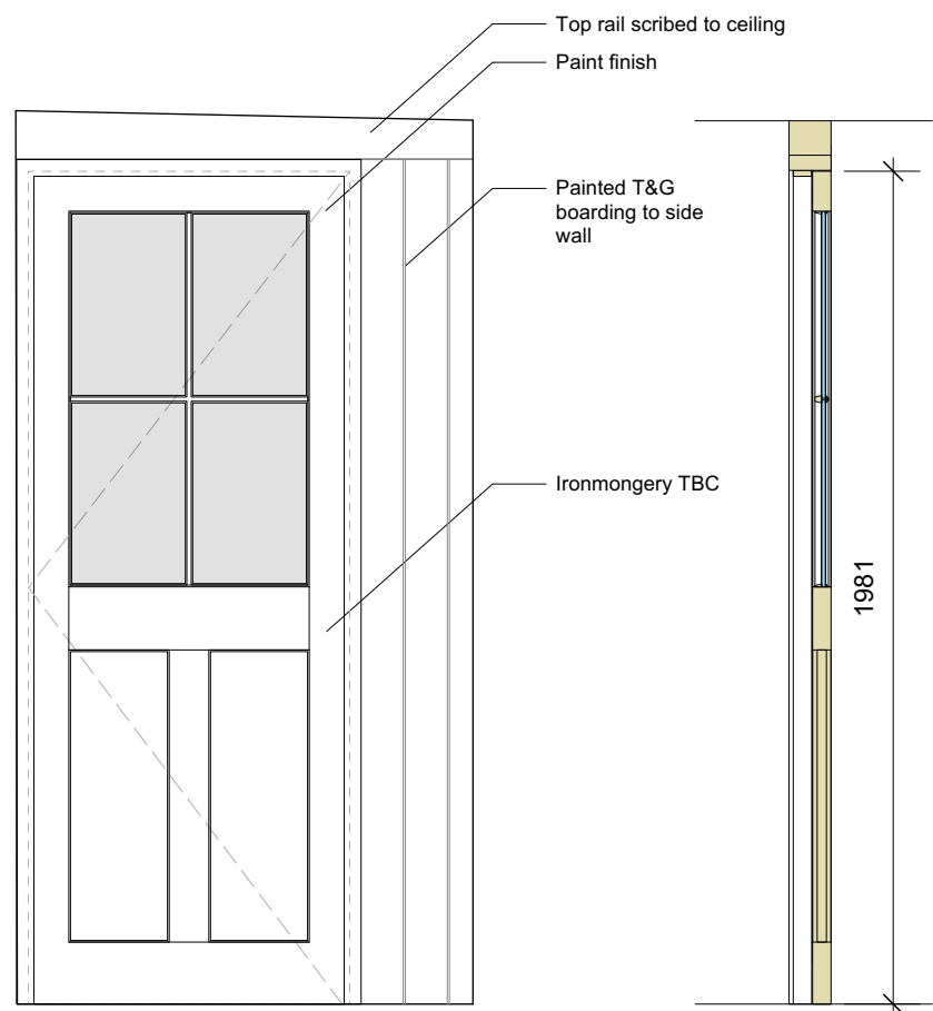
Door to Office D04 1:20 Elevation (Hallway side)
