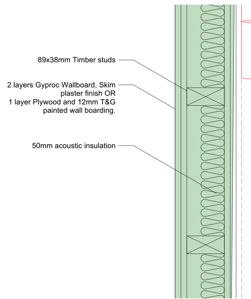
New Internal Wall Partitions Plan Details 1:5
