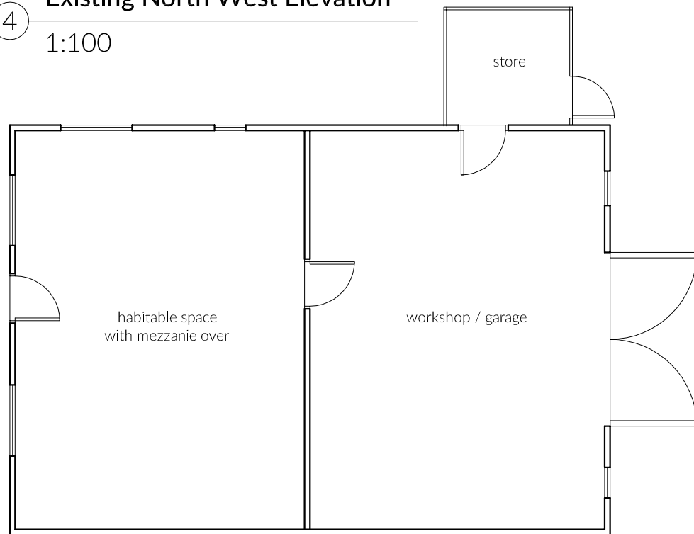
1 Existing Ground Floor Plan 1:100
