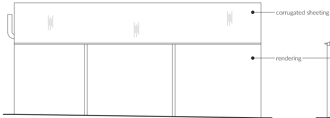
2 Existing South East Elevation 1:100
