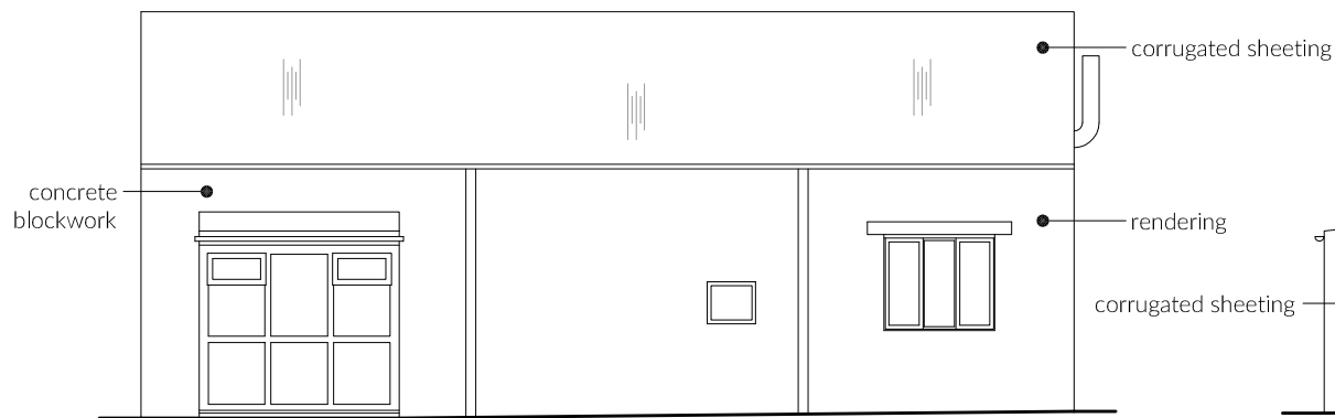
4 Existing North West Elevation 1:100
