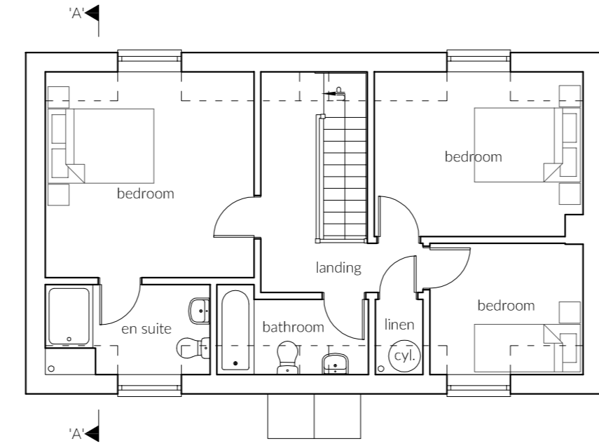
2 Proposed First Floor Plan 1:100
