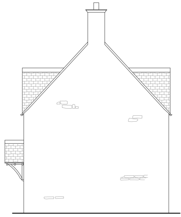
4 Proposed North West Elevation 1:100
