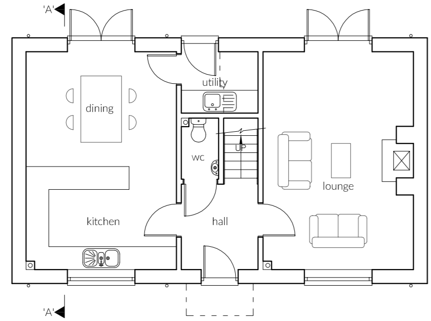
1 Proposed Ground Floor Plan 1:100
