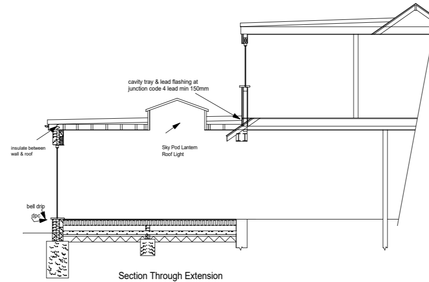
Section Through Extension
