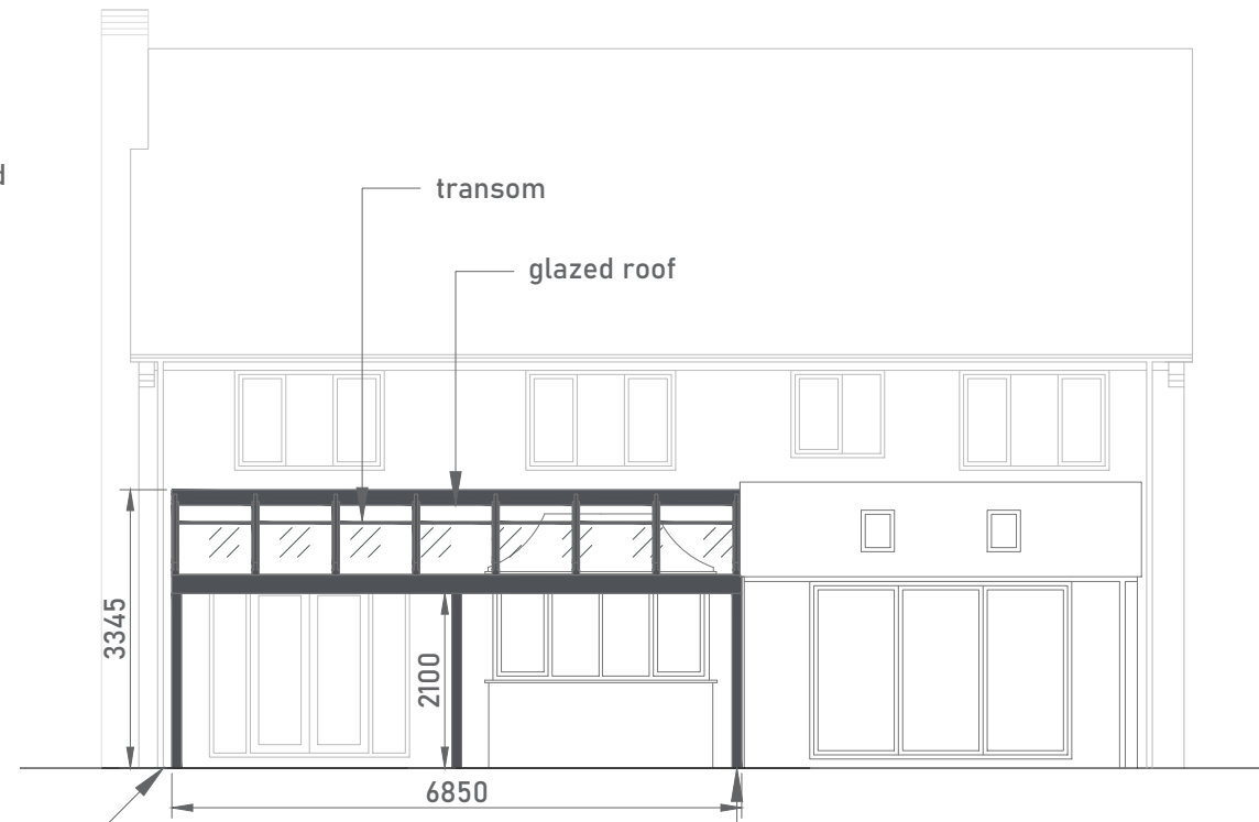
REAR ELEVATION
