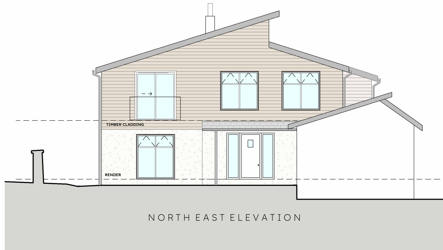
1 - ELEVATIONS NW & NE - PROPOSED 1 : 100
