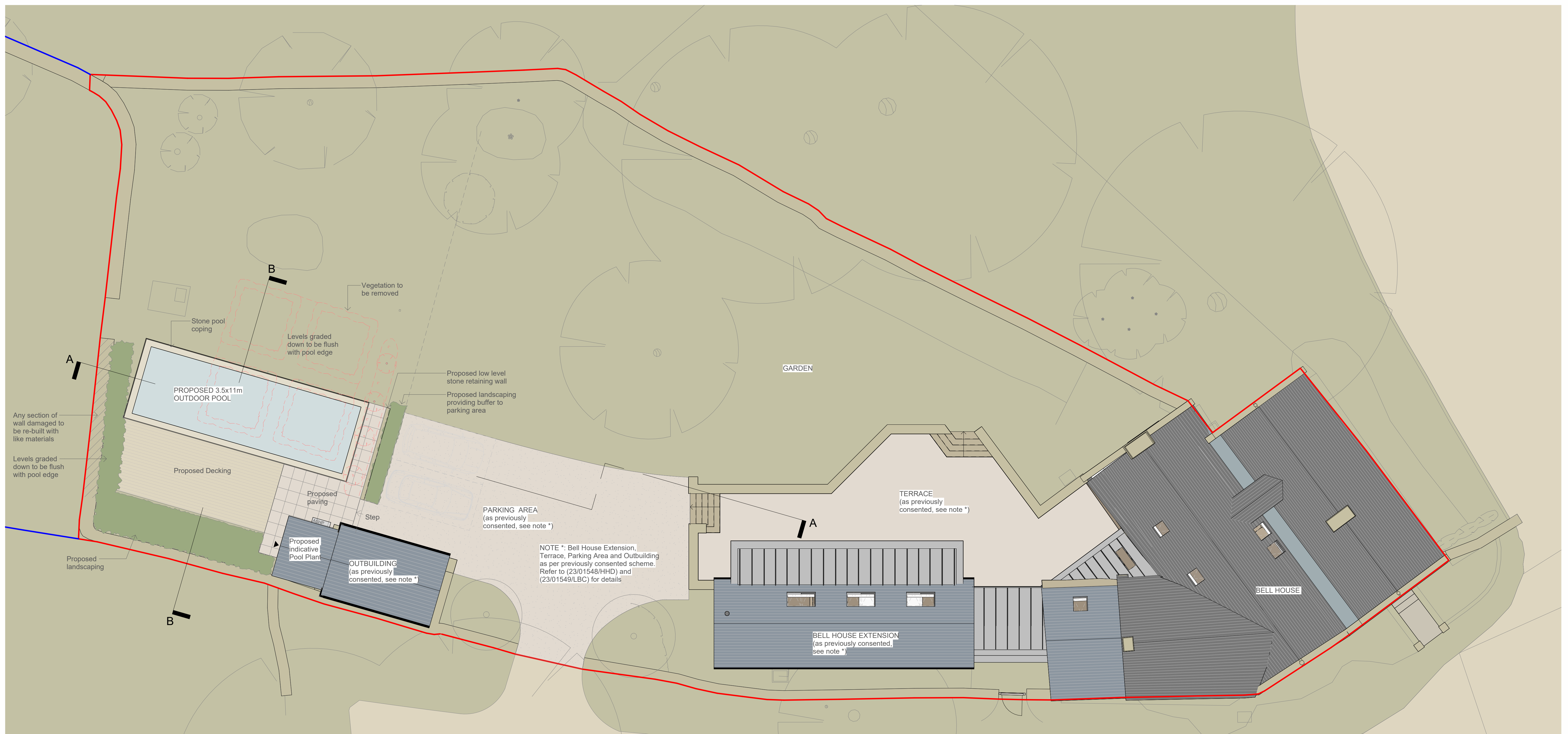
Outdoor Pool Plan 1:100
