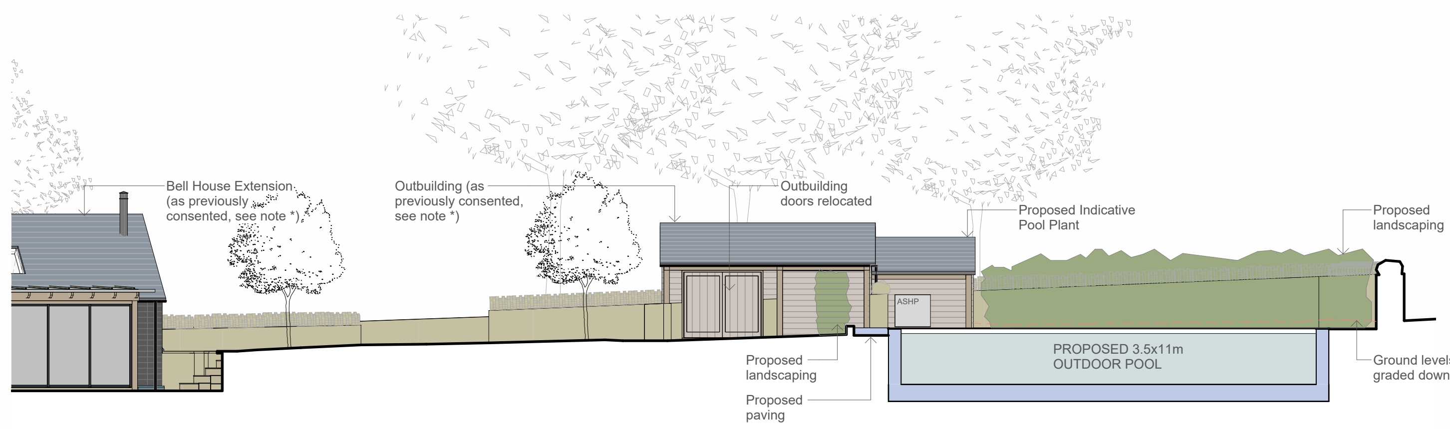
Outdoor Pool Section A 1:100
