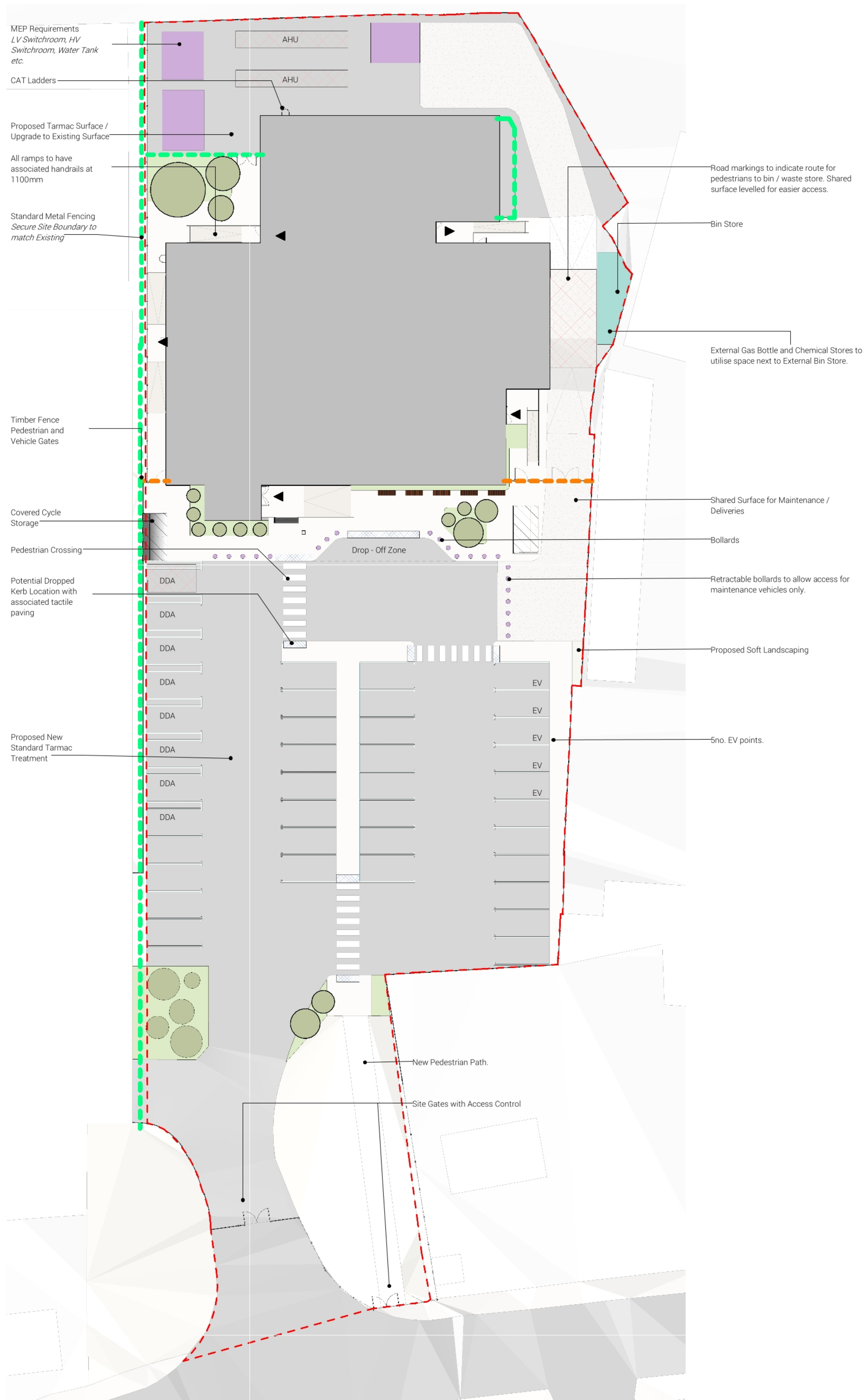
Proposed External Works Plan 1:200
