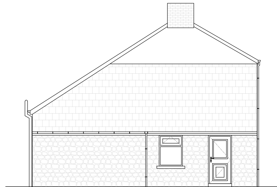
EXISTING NORTH EAST ELEVATION 1:100
