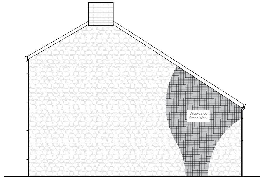
EXISTING SOUTH WEST ELEVATION 1:100
