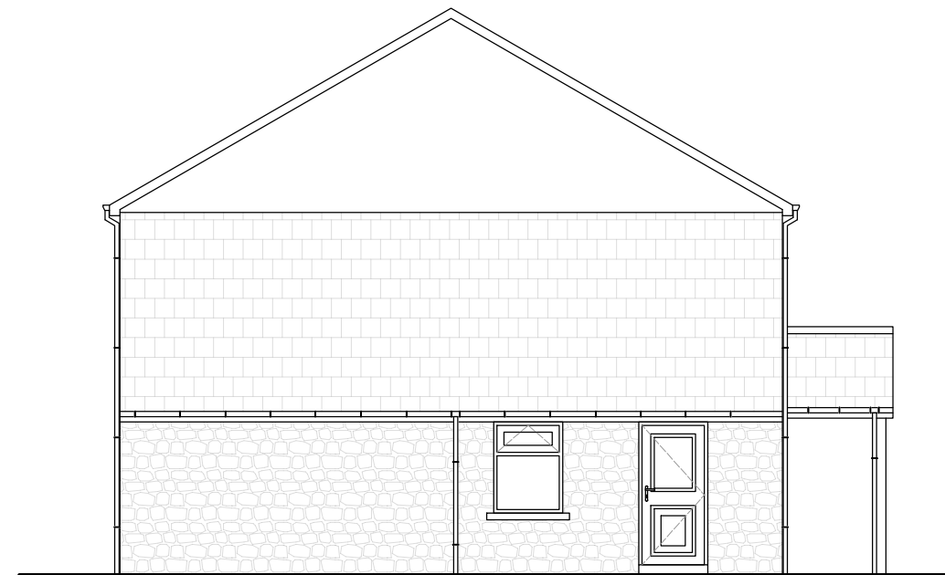
PROPOSED NORTH EAST ELEVATION 1:100
