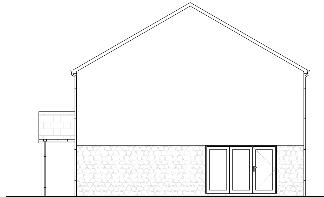
PROPOSED SOUTH WEST ELEVATION 1:100
