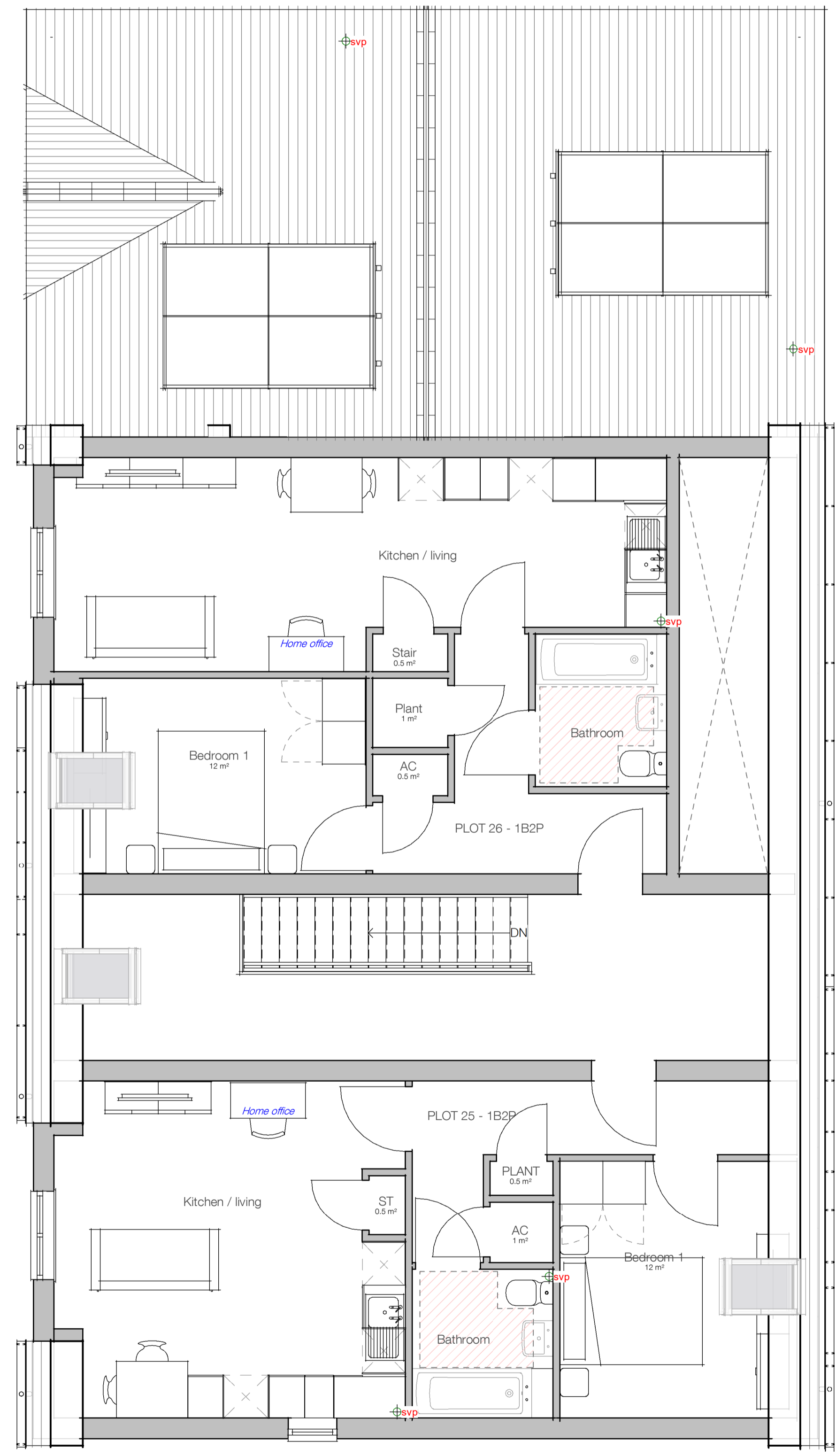
Block 2 - Second floor 1 : 50
