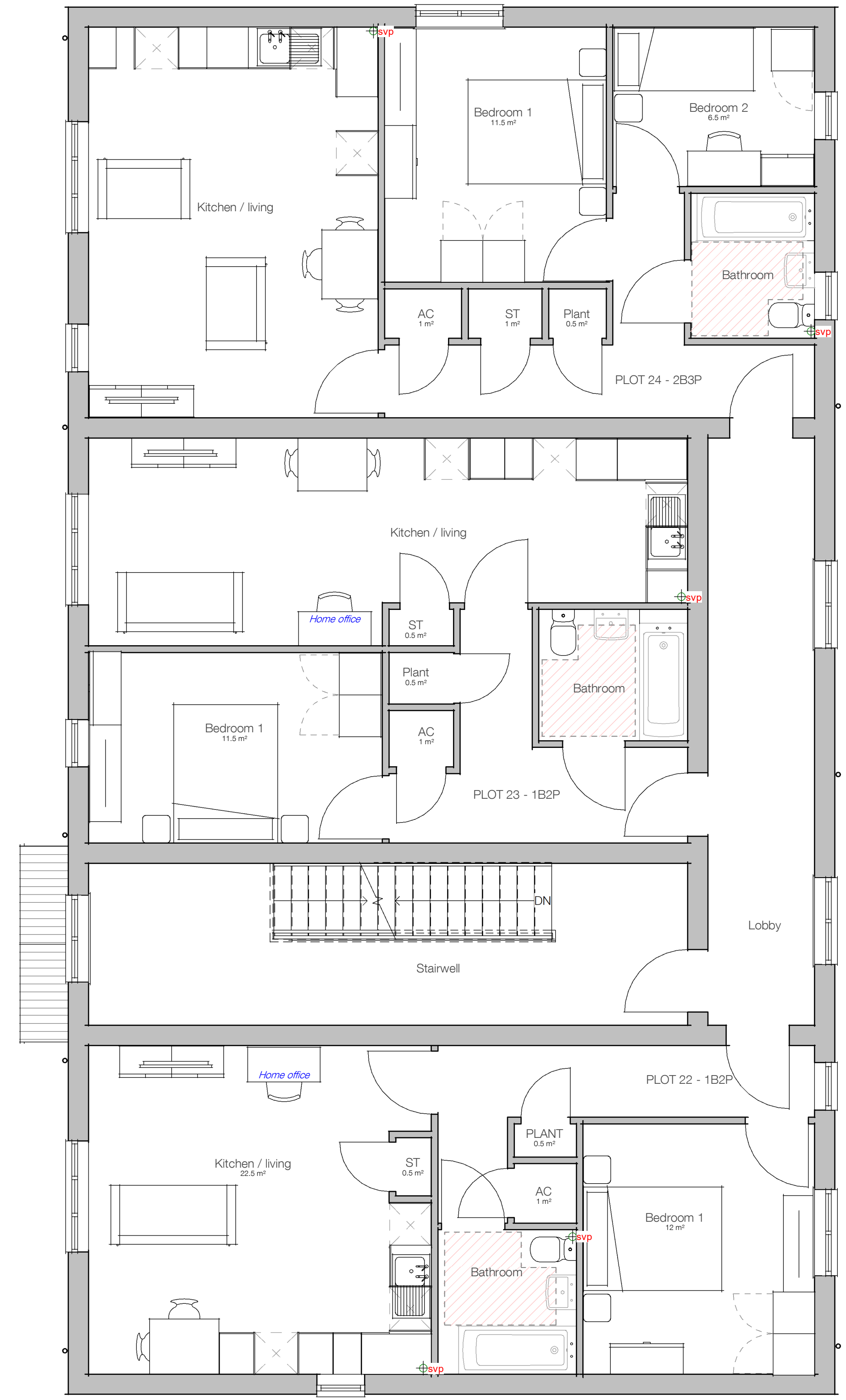
Block 2 - First floor plan 1 : 50
