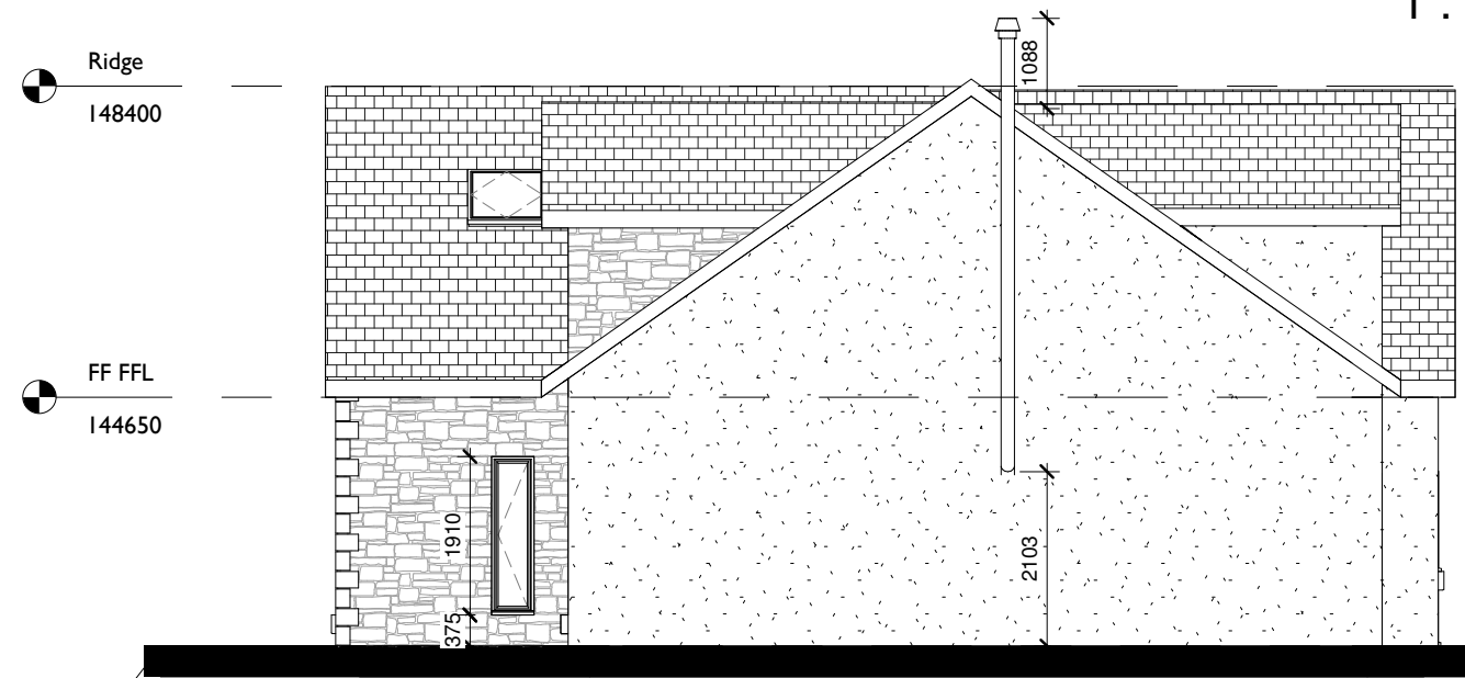
Gable Elevation 1 : 100
