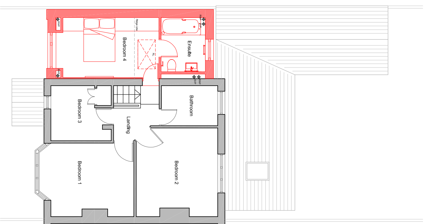
03. Proposed First Floor Plan
