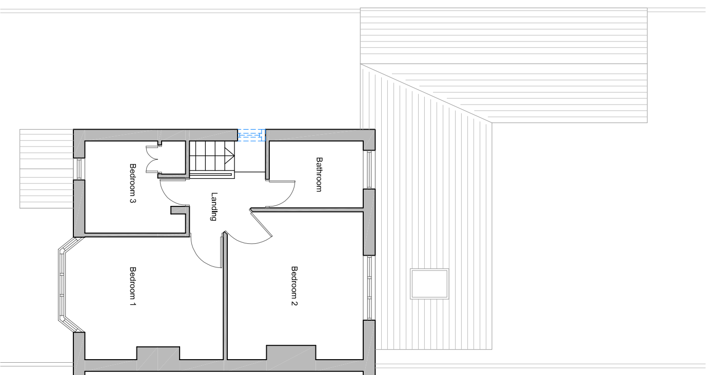
02. Demolition First Floor Plan
