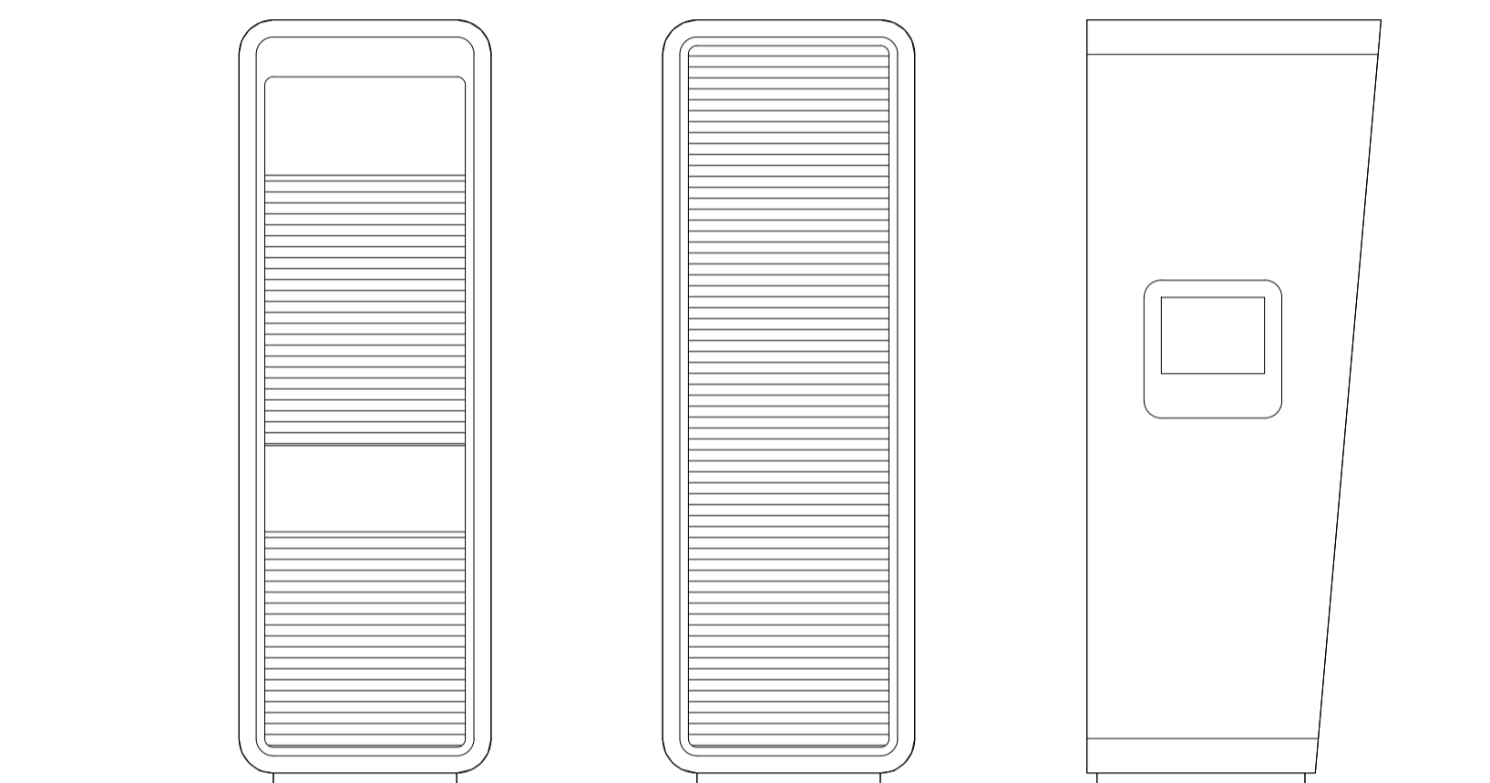
FRONT ELEVATION BACK ELEVATION SIDE ELEVATION CHARGING UNIT Scale 1:20
