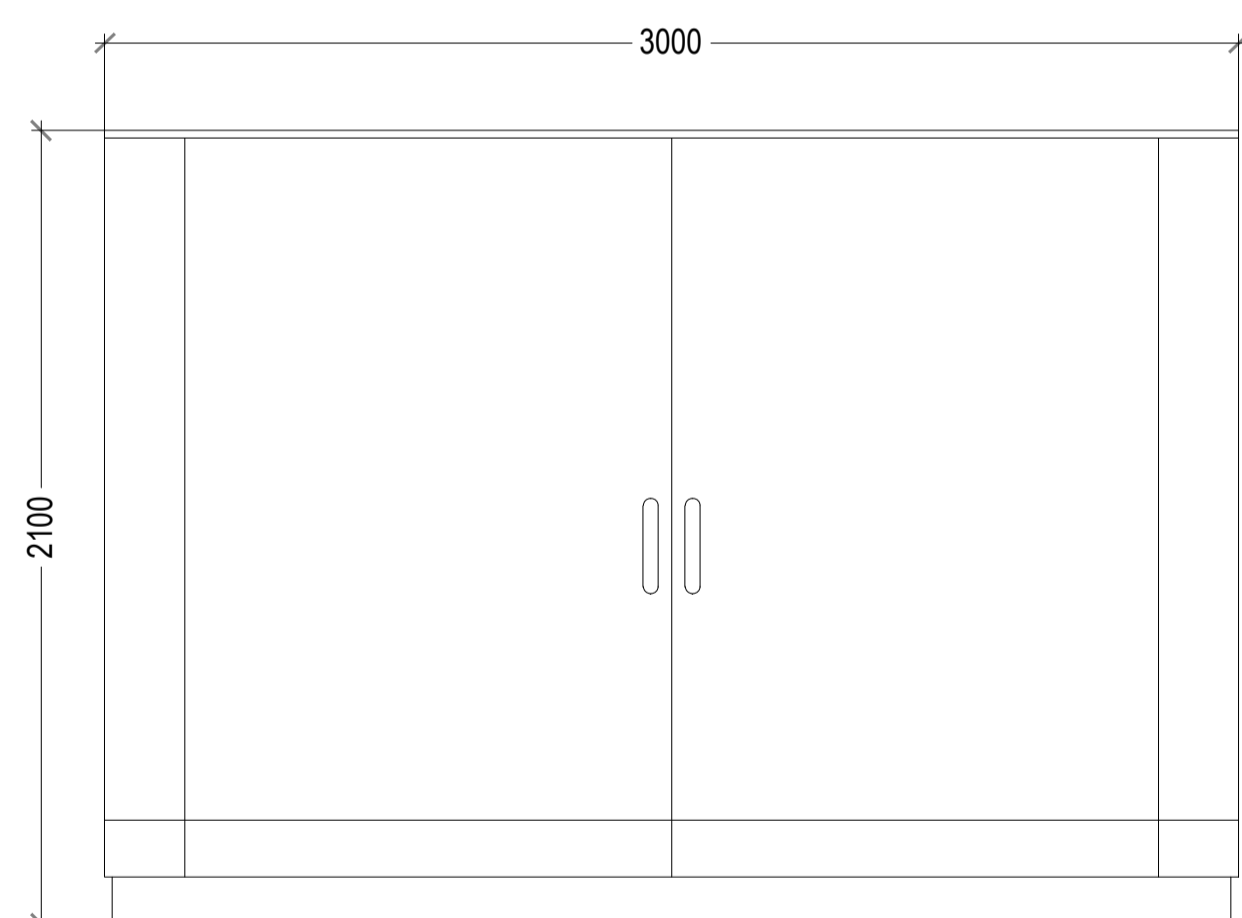
Front Elevation
