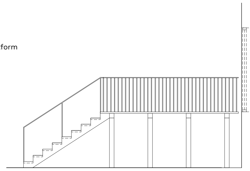
2 PROPOSED ELEVATION AA 1:50 / A3
