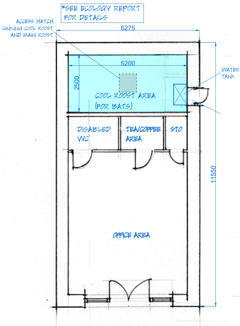
FLOOR PLAN
