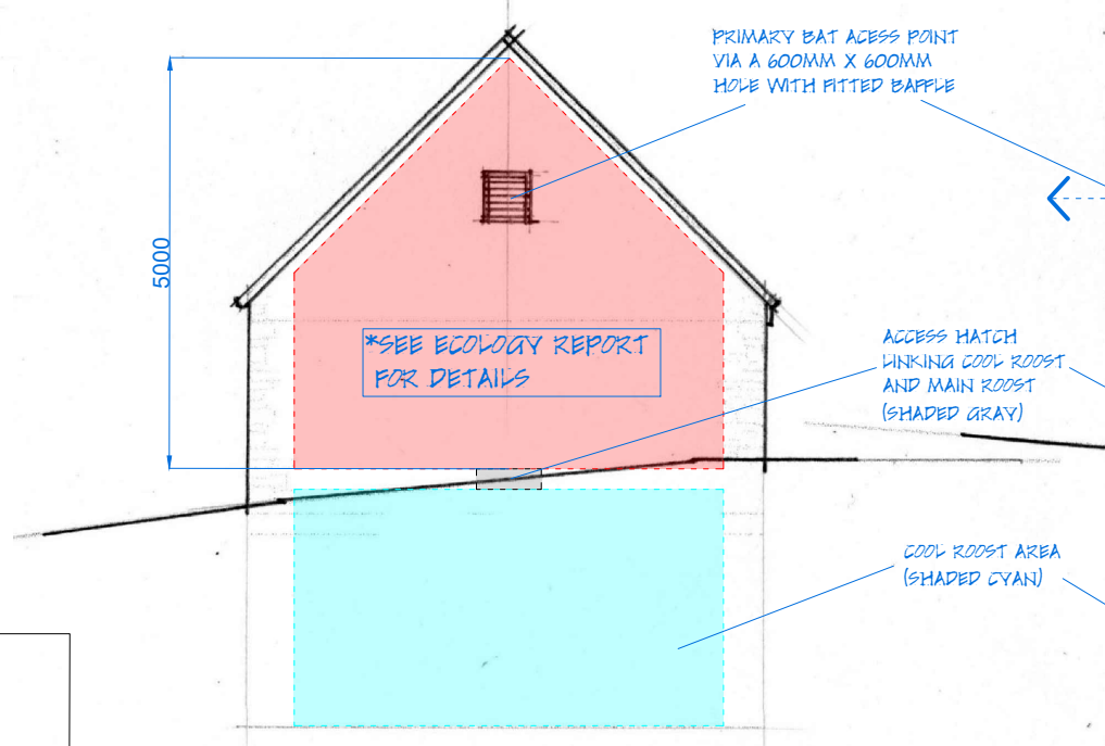
NORTH ELEVATION
