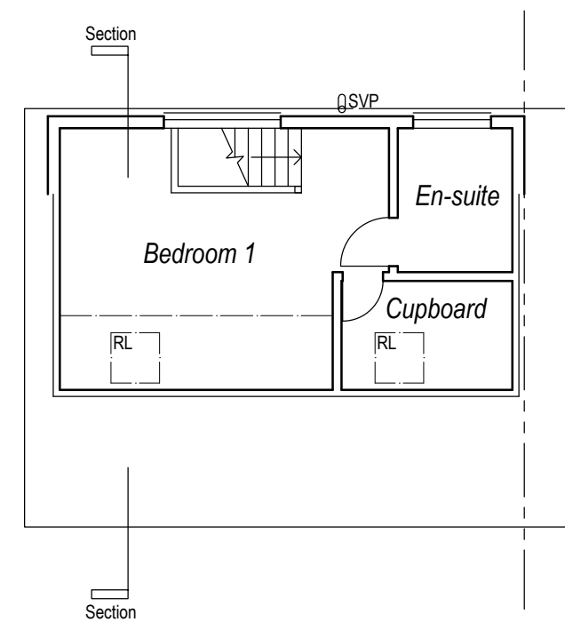
Roof Plan @ 1:100
