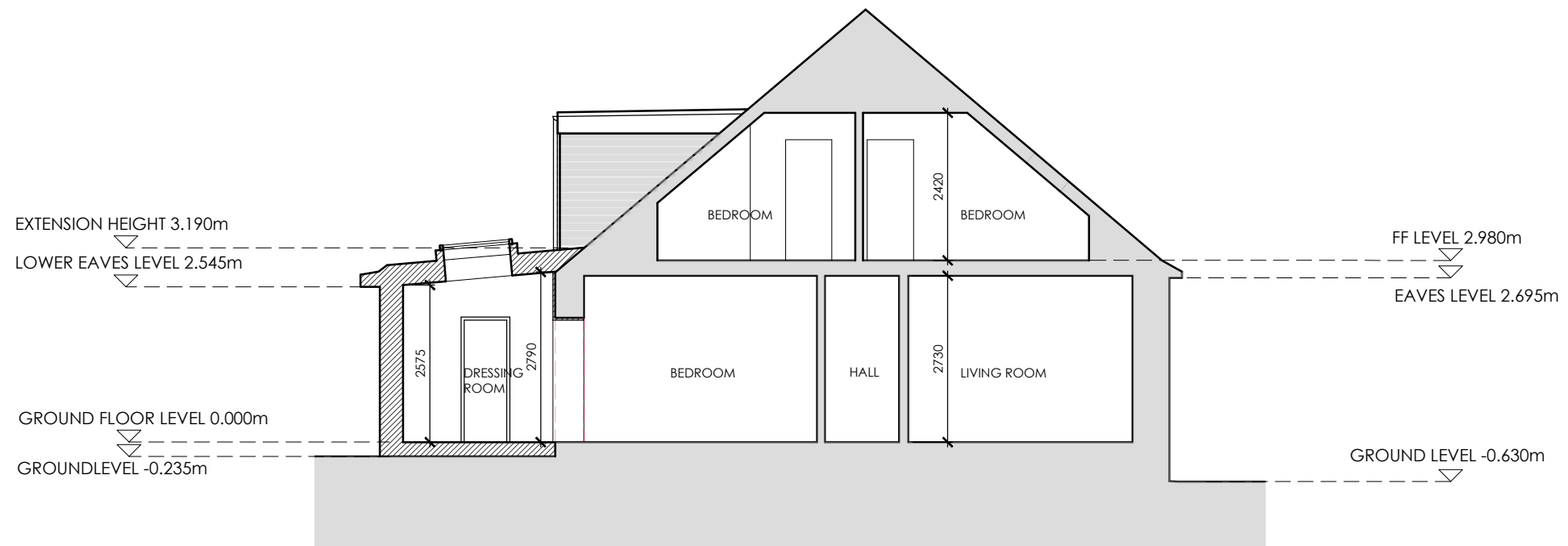
SECTION A-A AS PROPOSED
