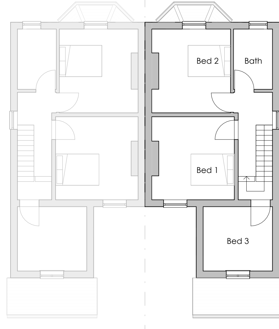
First Floor
