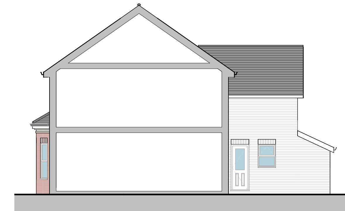
West Elevation
