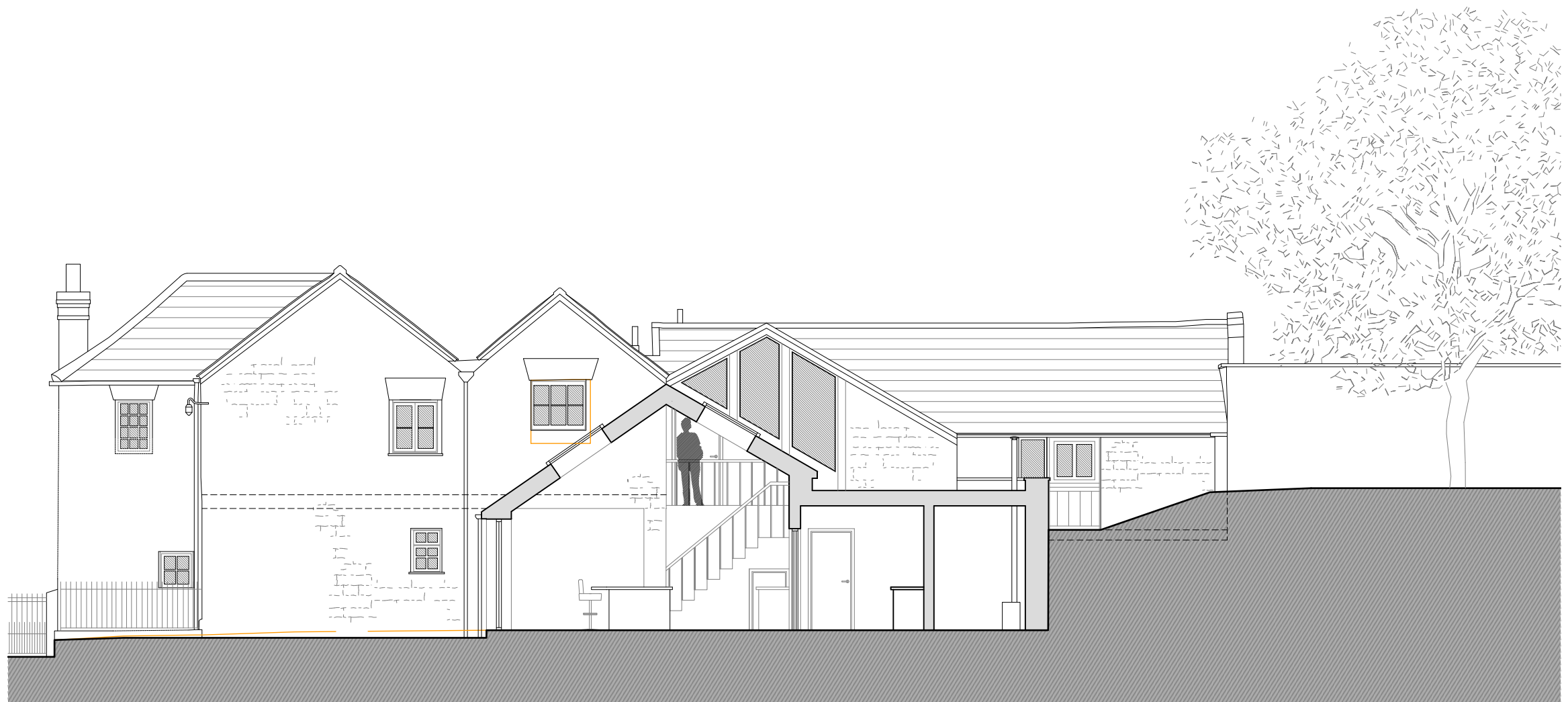
Section BB
