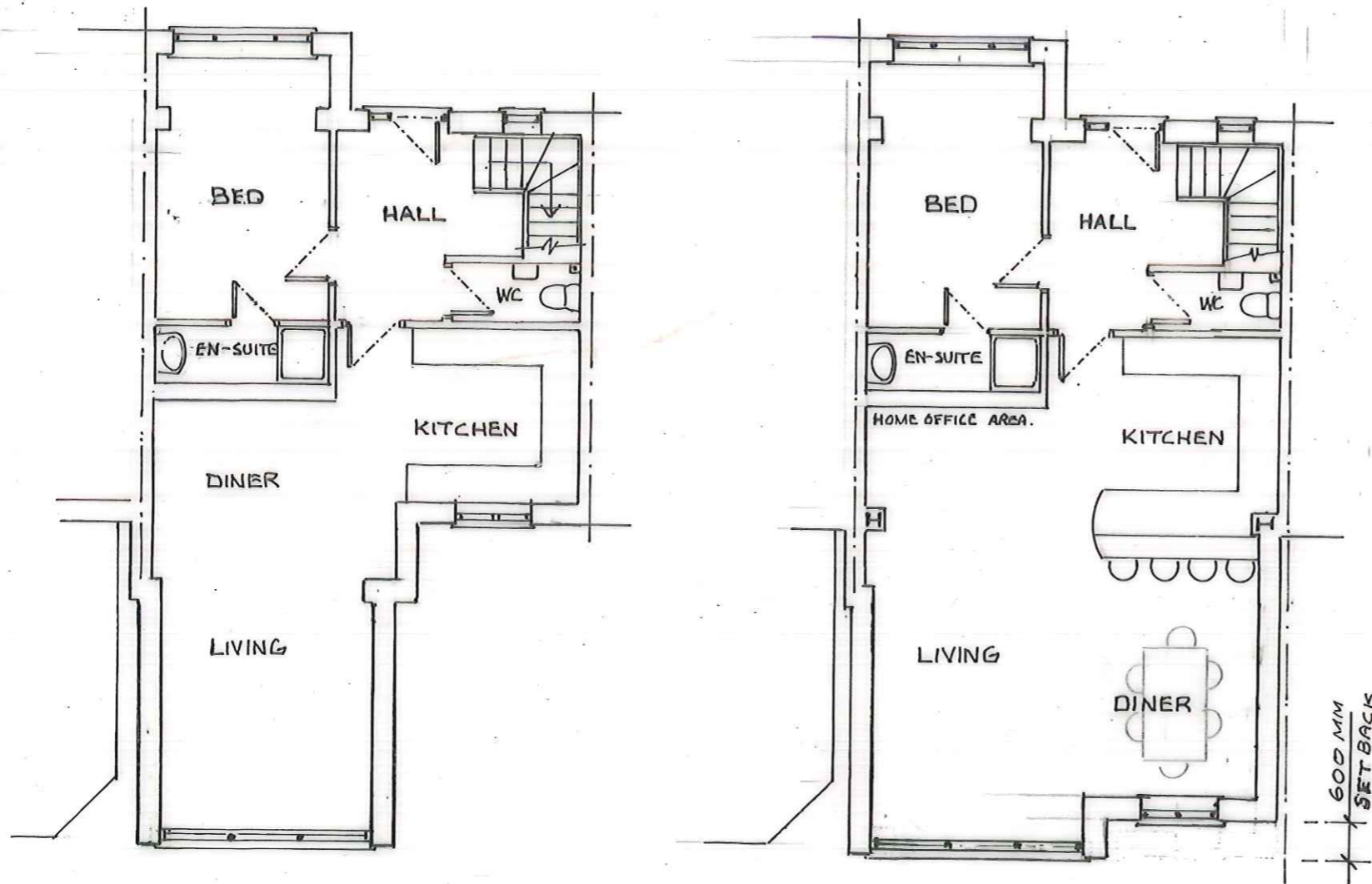
EXISTING GRD. FLR. PLAN 1:100 PROPOSED GRD. FLR. PLAN
