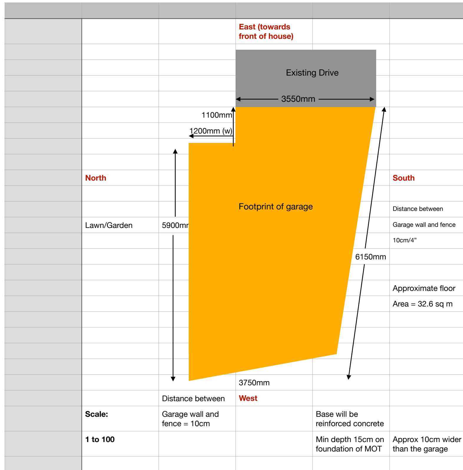
Figure 1. Footprint of Garage - 52 High Street Cottenham
